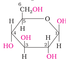
\beta -D-(+)-Glucopyranose
