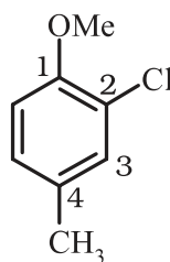
2-Chloro-4-methylanisole
