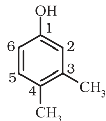
3,4-Dimethylphenol
