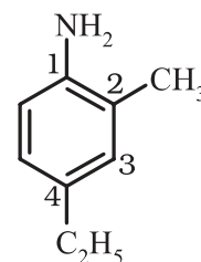
4-Ethyl-2-methylaniline
