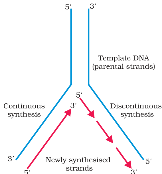
Figure 5.8 Replicating Fork
