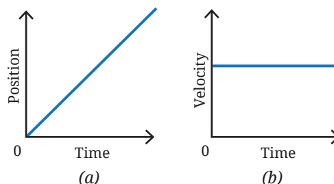
Fig. 6.16: When the object is moving with a constant velocity, its (a) position-time graph, (b) velocity-time graph
