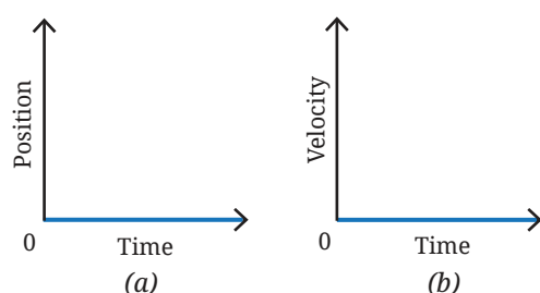
Fig. 6.15: When the object is at rest, its (a) position-time graph, (b) velocity-time graph
