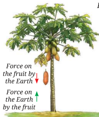
Fig. 6.33: The Earth and the fruit applying equal and opposite gravitational forces on each other
