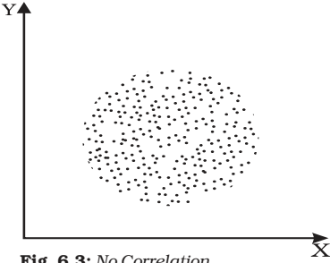
Fig. 6.3: No Correlation
