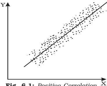
Fig. 6.1: Positive Correlation
