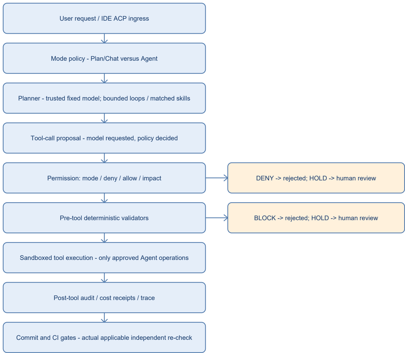
Figure 1. Agent execution control plane
