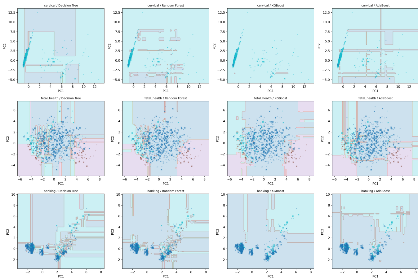
Figure 3: PCA decision-boundary visualizations.
