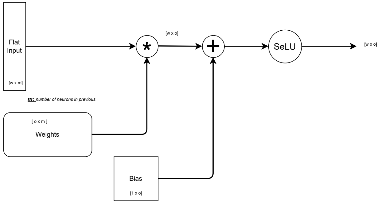
Mid Layer (this.prev, & this.next are FCN)
