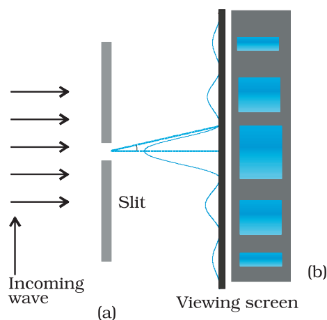
FIGURE 10.15 Intensity distribution and photograph of fringes due to diffraction at single slit.
