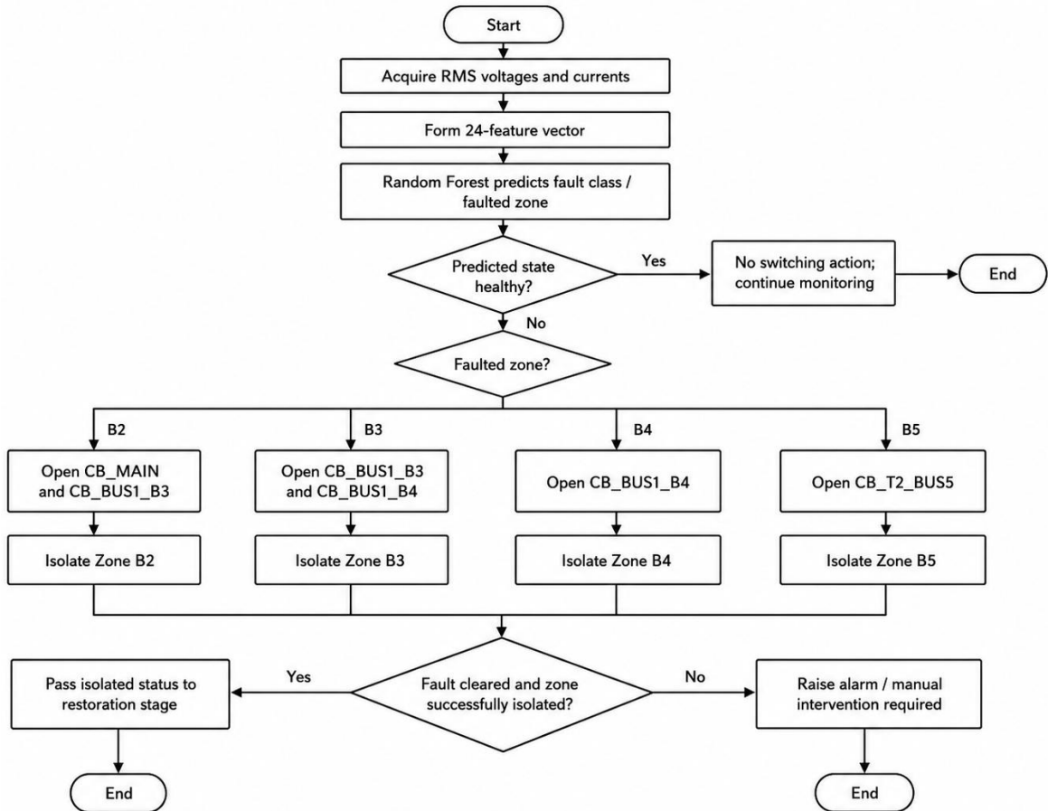
Figure 3.6: Selective fault-isolation logic
