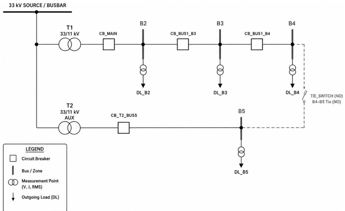
Figure 3.3: Single-line diagram of the five-bus feeder
