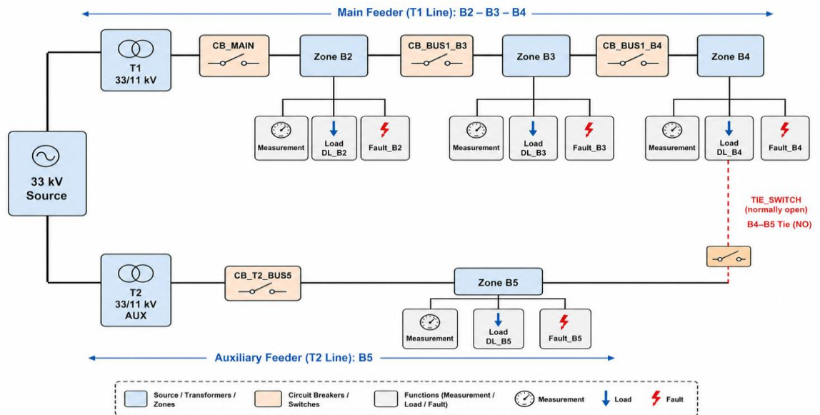
Figure 3.2: Feeder topology block diagram
