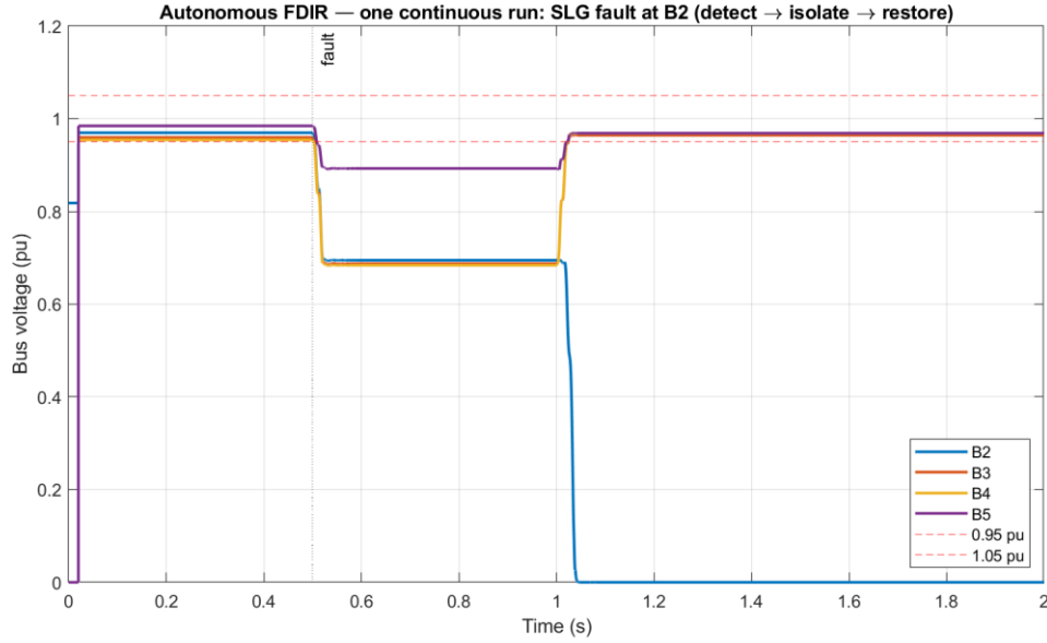
Figure 5.15: Autonomous FDIR operation in a single continuous simulation. An SLG fault at B2 ( t = 0.5 s) is detected, classified as SLG-B2 at t = 1.001 s, isolated ( B2 to 0 pu), and the healthy buses restored through the tie ( \sim 0.97 pu) by t \sim 1.03 s.
