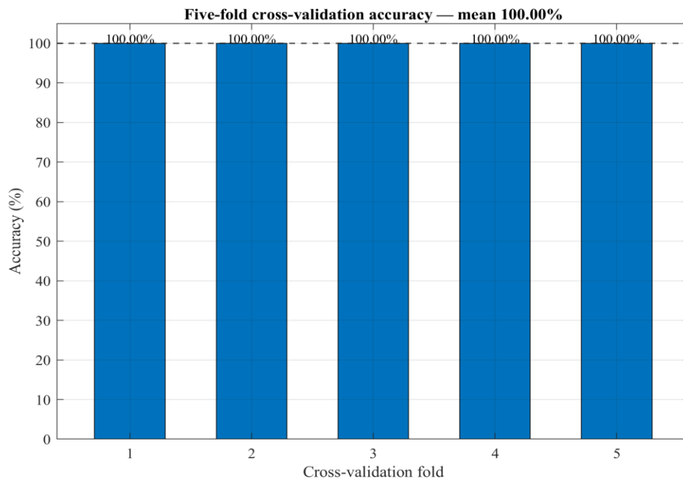
Figure 5.10: Five-fold cross-validation accuracy
