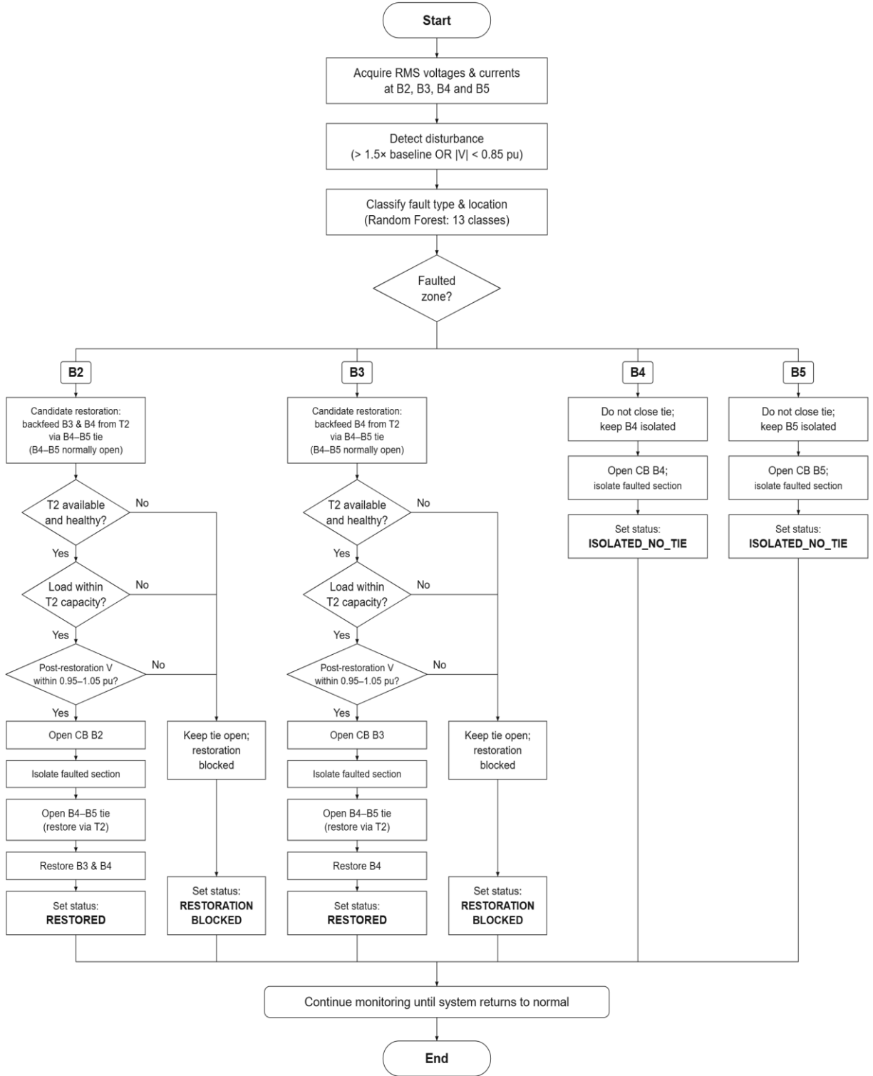
Figure 3.7: Self-healing restoration logic
