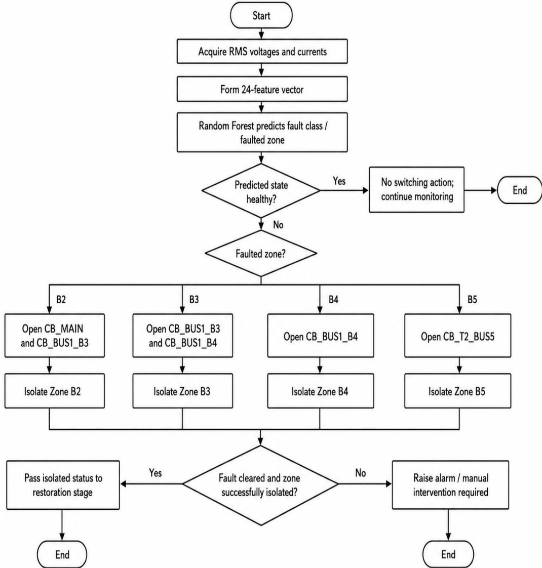
Figure 3.6: Selective fault-isolation logic
