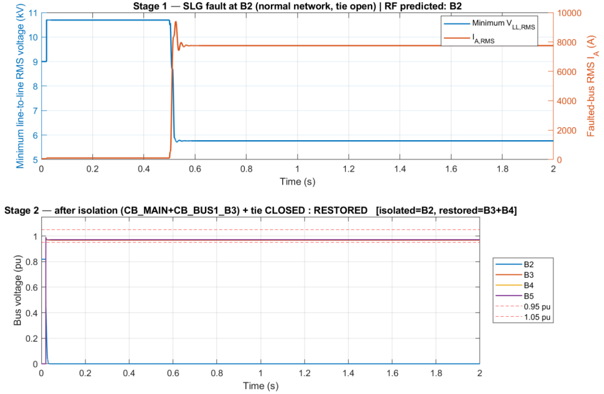
Figure 5.3: SLG fault at B2 - fault and restoration waveforms
