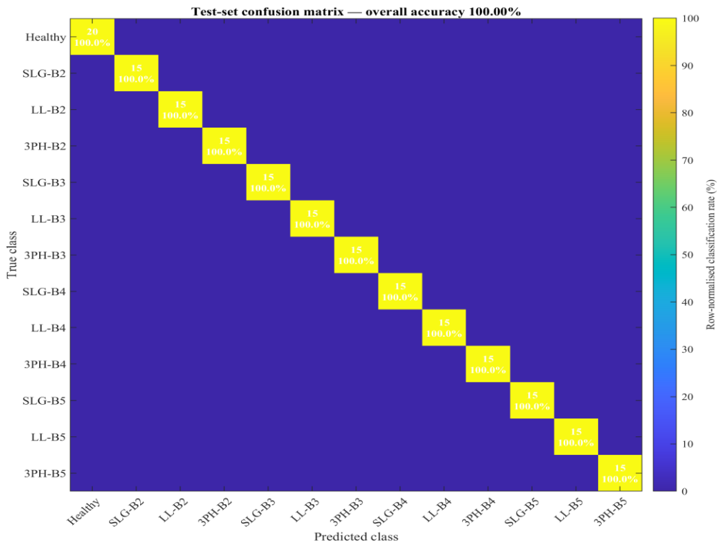
Figure 5.8: Test-set confusion matrix
