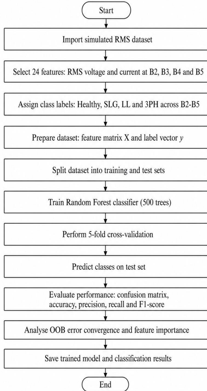
Figure 3.5: Machine-learning training pipeline
