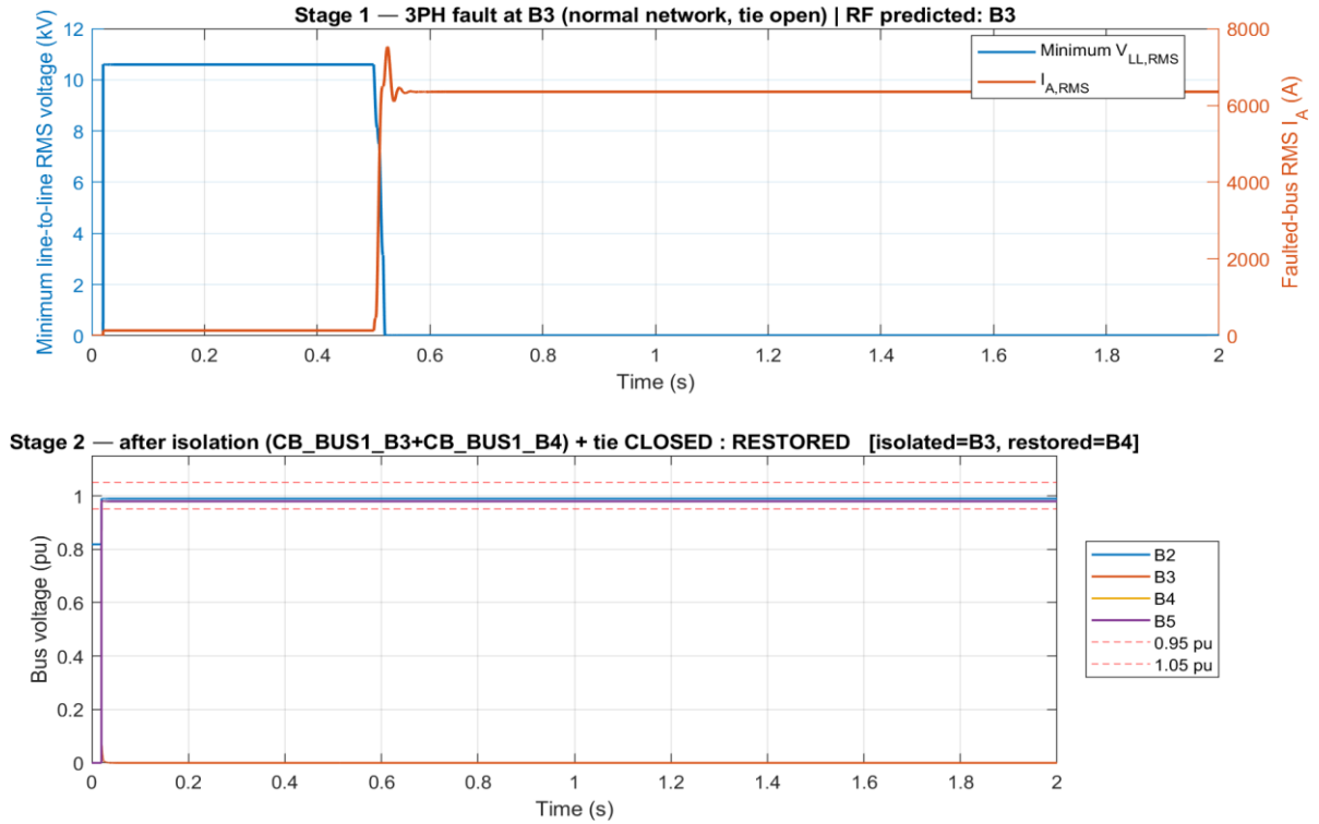
Figure 5.4: Three-phase fault at B3 - fault and restoration waveforms
