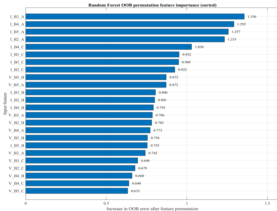
Figure 5.11: OOB permutation feature importance
