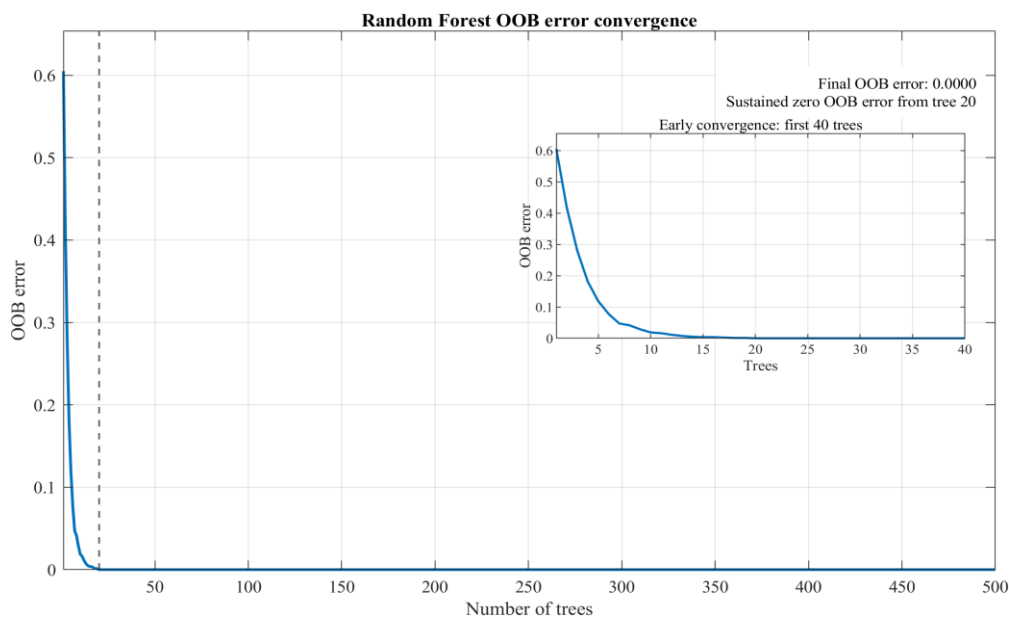
Figure 5.7: Random Forest out-of-bag error convergence
