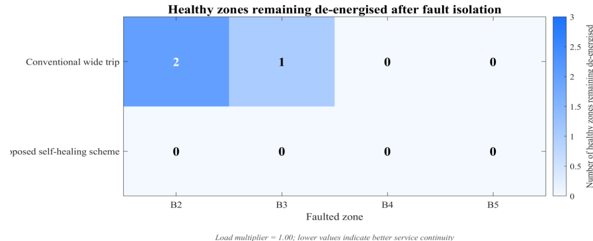
Figure 6.1: Healthy zones remaining de-energised after fault isolation
