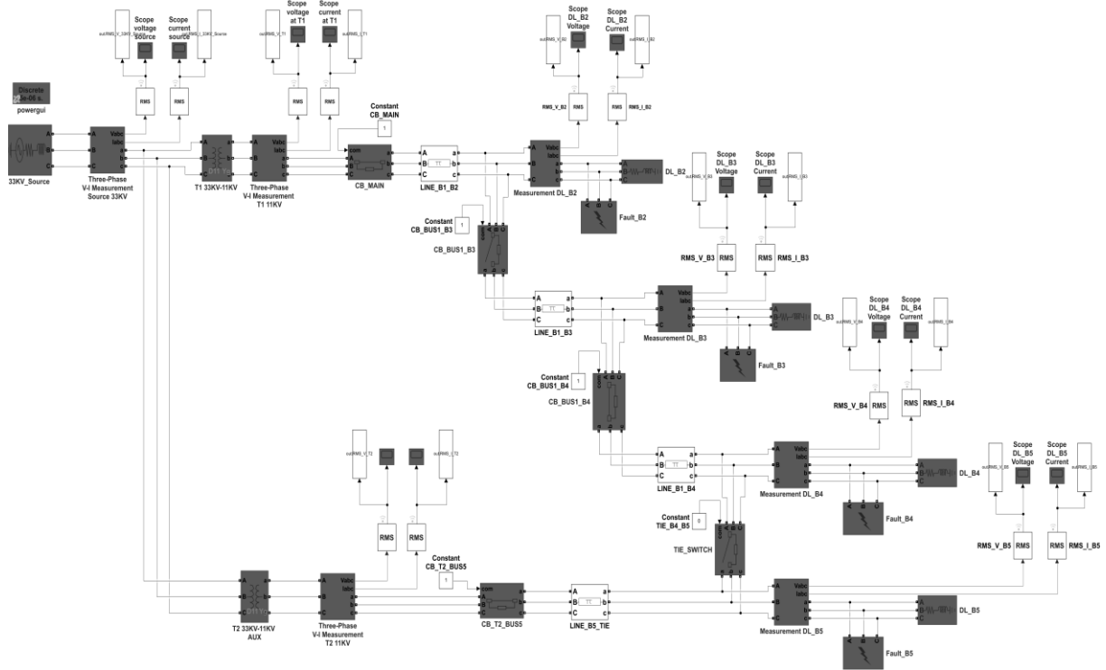
Figure 4.1: Simulink feeder model canvas
