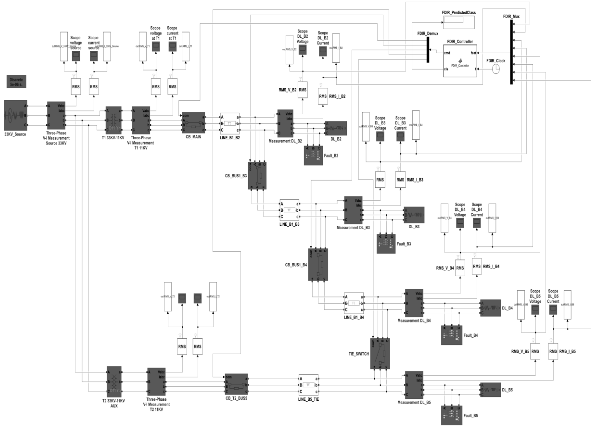
Figure 4.5: Final feeder model with the autonomous in-model FDIR controller. The added blocks (top-right) are the feature Mux, the MATLAB Function controller, the Clock, the command Demux and the predicted-class display; their five outputs drive the breaker and tie-switch control inputs.
