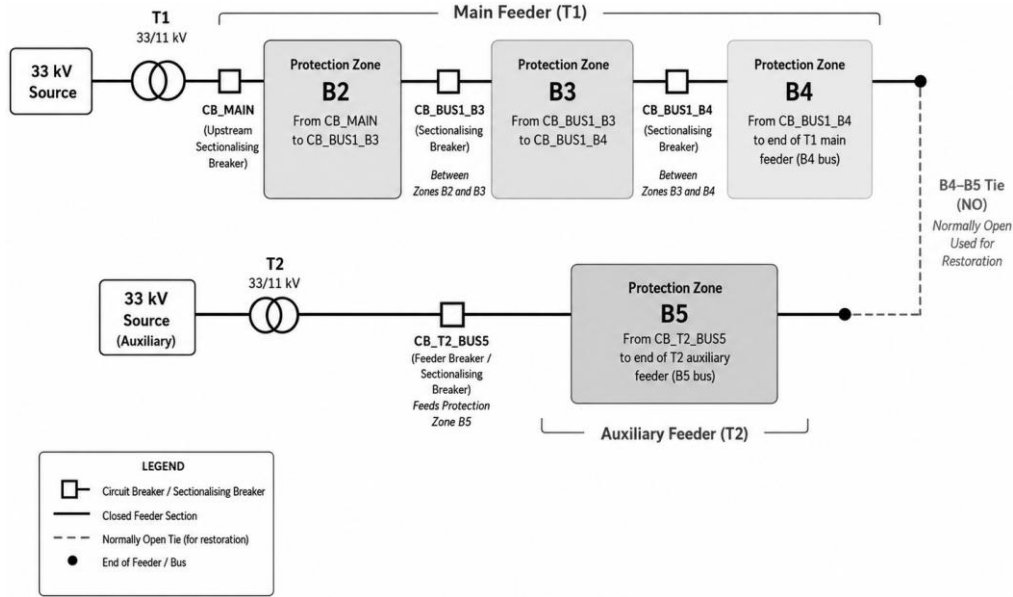
Figure 3.4: Protection zones and the normally-open tie
