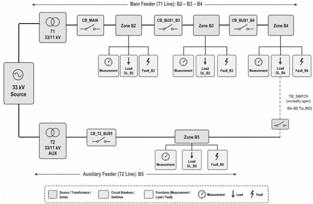
Figure 3.2: Feeder topology block diagram
