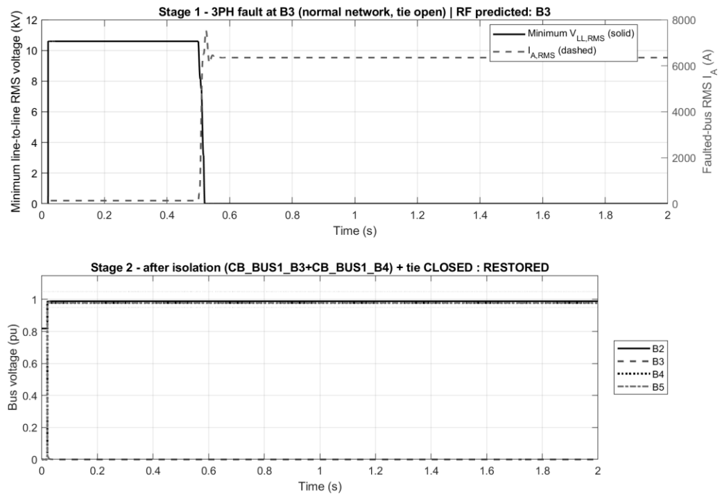
Figure 5.4: Three-phase fault at B3 - fault and restoration waveforms
