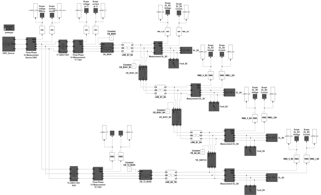
Figure 4.1: Simulink feeder model canvas
