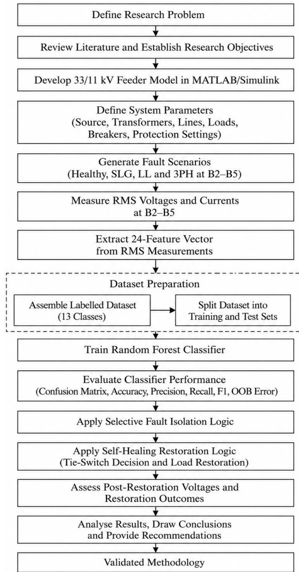
Figure 3.1: Research methodology workflow
