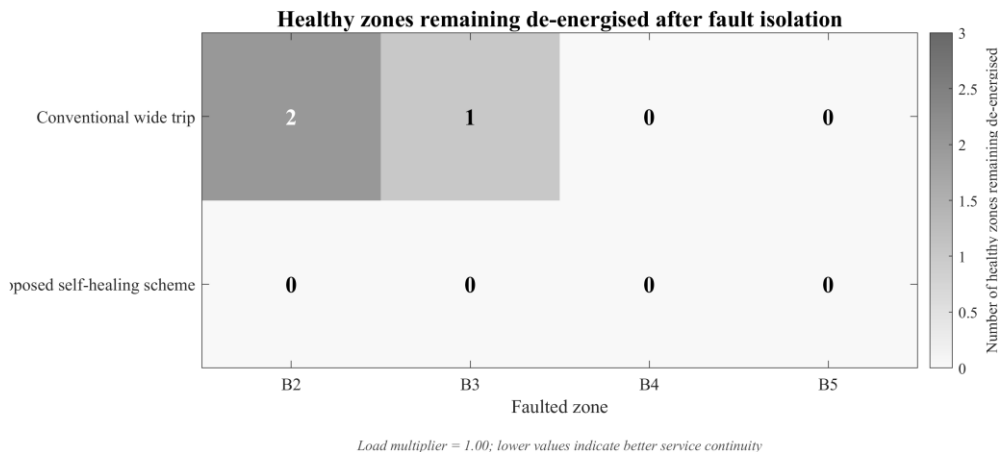
Figure 6.1: Healthy zones remaining de-energised after fault isolation
