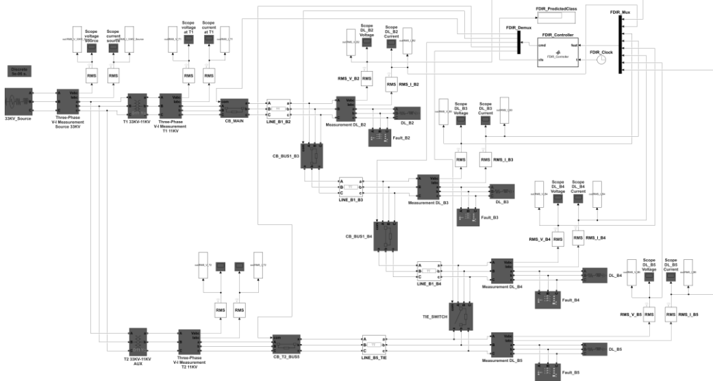
Figure 4.5: Final feeder model with the autonomous in-model FDIR controller. The added blocks (top-right) are the feature Mux, the MATLAB Function controller, the Clock, the command Demux and the predicted-class display; their five outputs drive the breaker and tie-switch control inputs.
