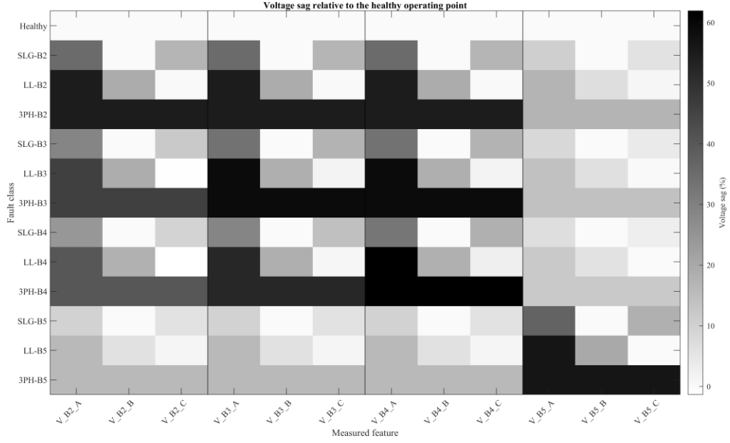
Figure 5.1: Per-class voltage signature (RMS)
