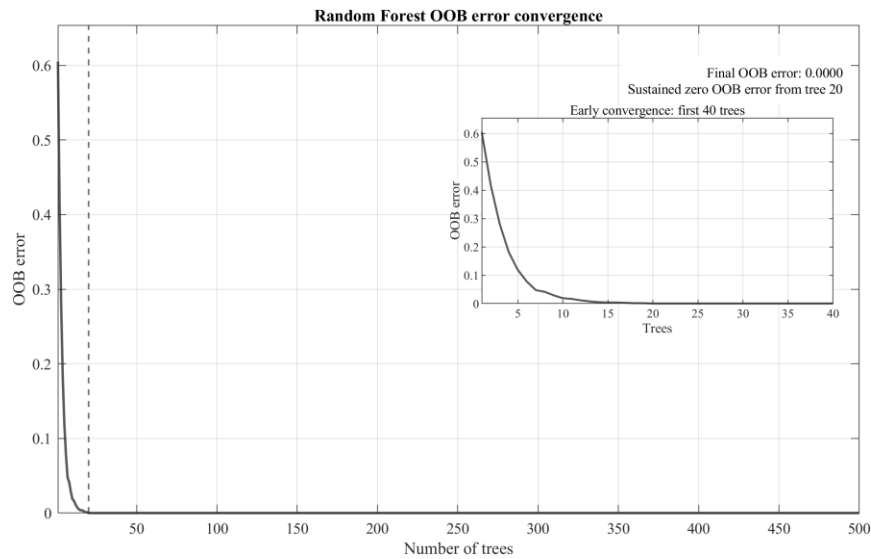
Figure 5.7: Random Forest out-of-bag error convergence
