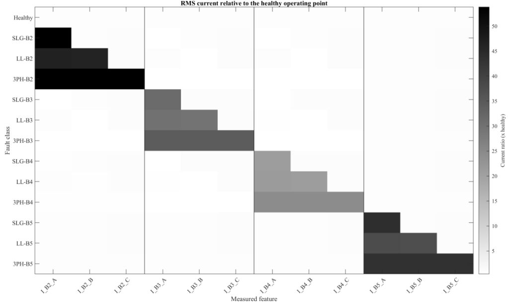
Figure 5.2: Per-class current signature (RMS)
