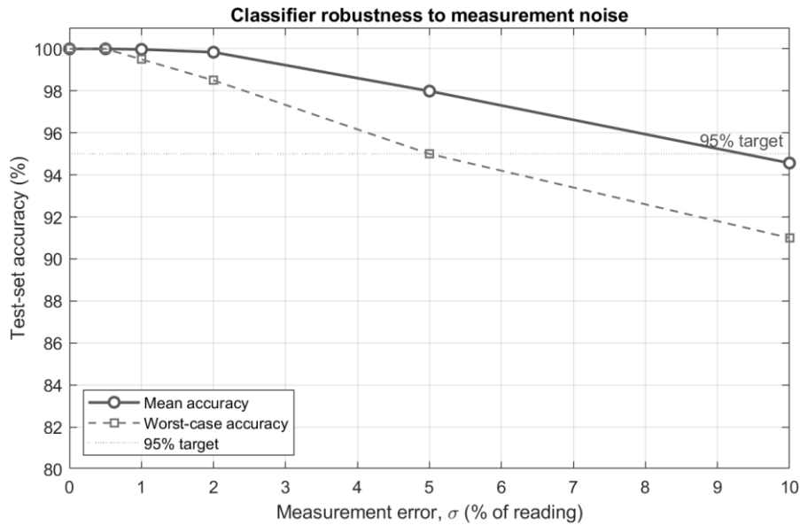
Figure 5.14: Classifier accuracy versus measurement noise
