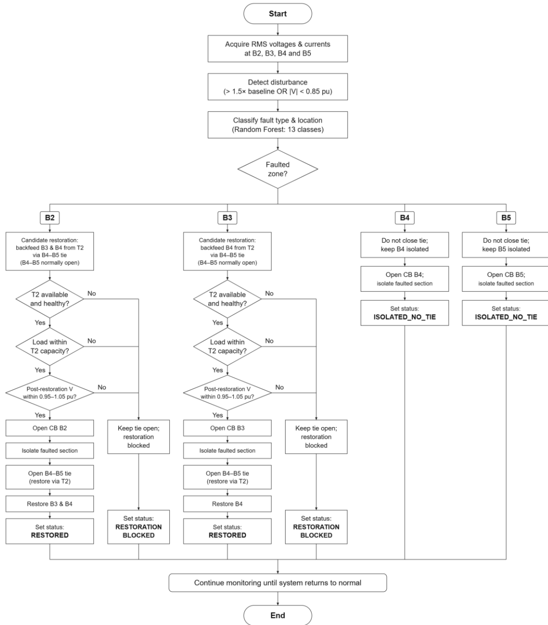
Figure 3.7: Self-healing restoration logic
