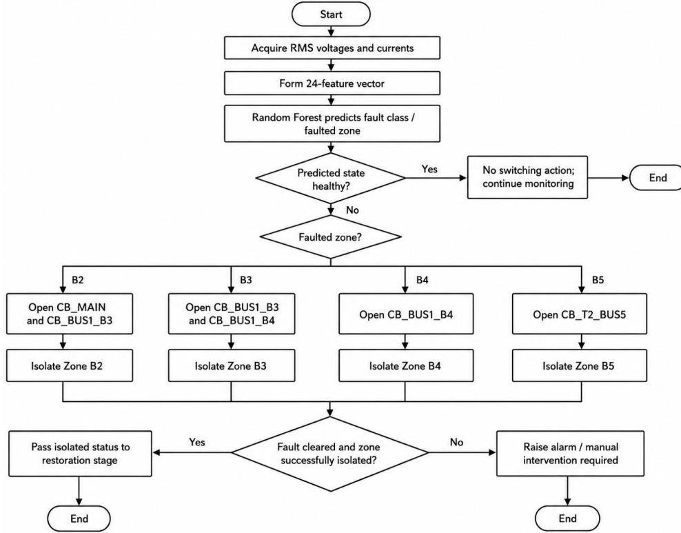
Figure 3.6: Selective fault-isolation logic
