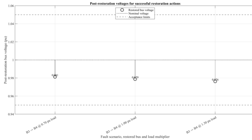
Figure 5.13: Post-restoration voltage - eligible (RESTORED) cases
