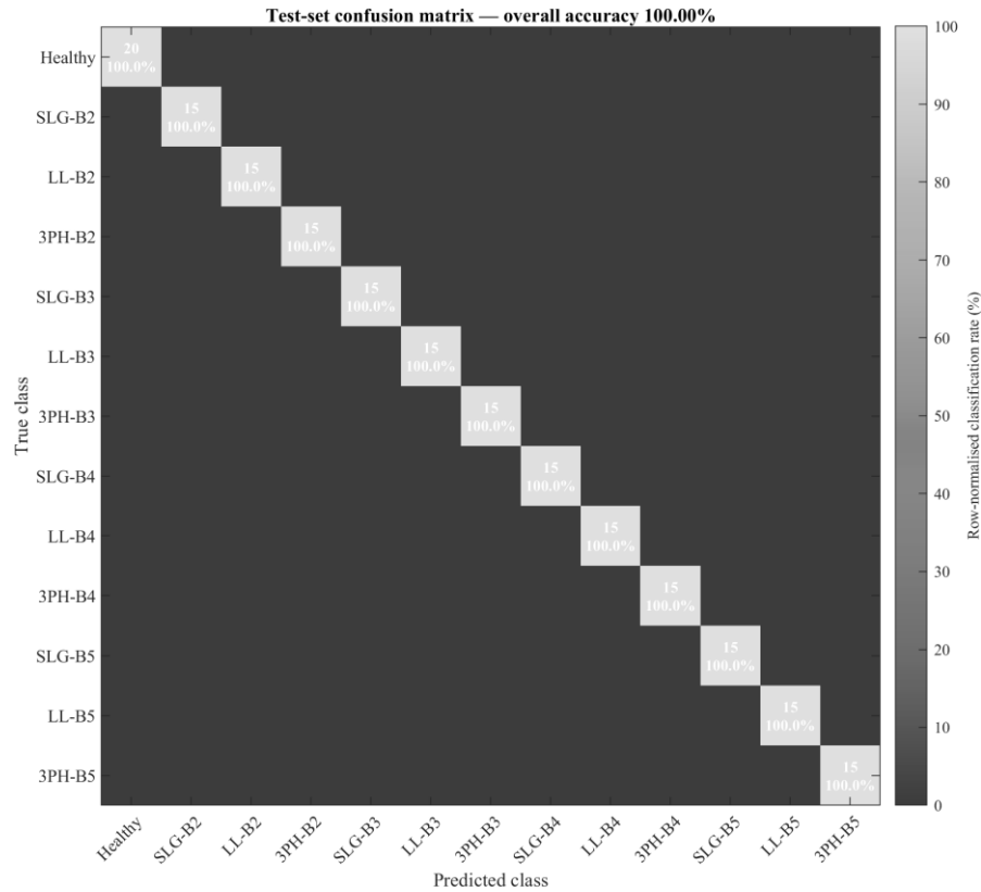
Figure 5.8: Test-set confusion matrix
