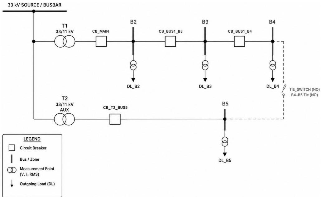
Figure 3.3: Single-line diagram of the five-bus feeder
