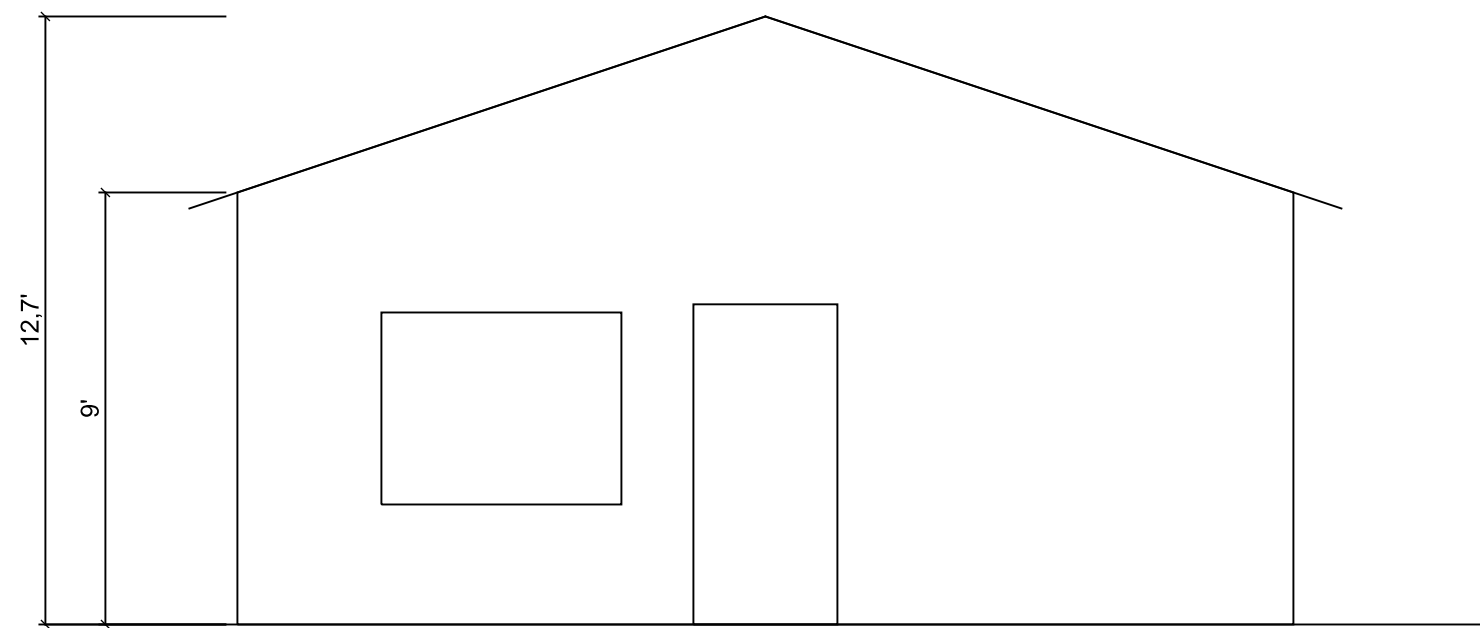
FRONT ELEVATION
