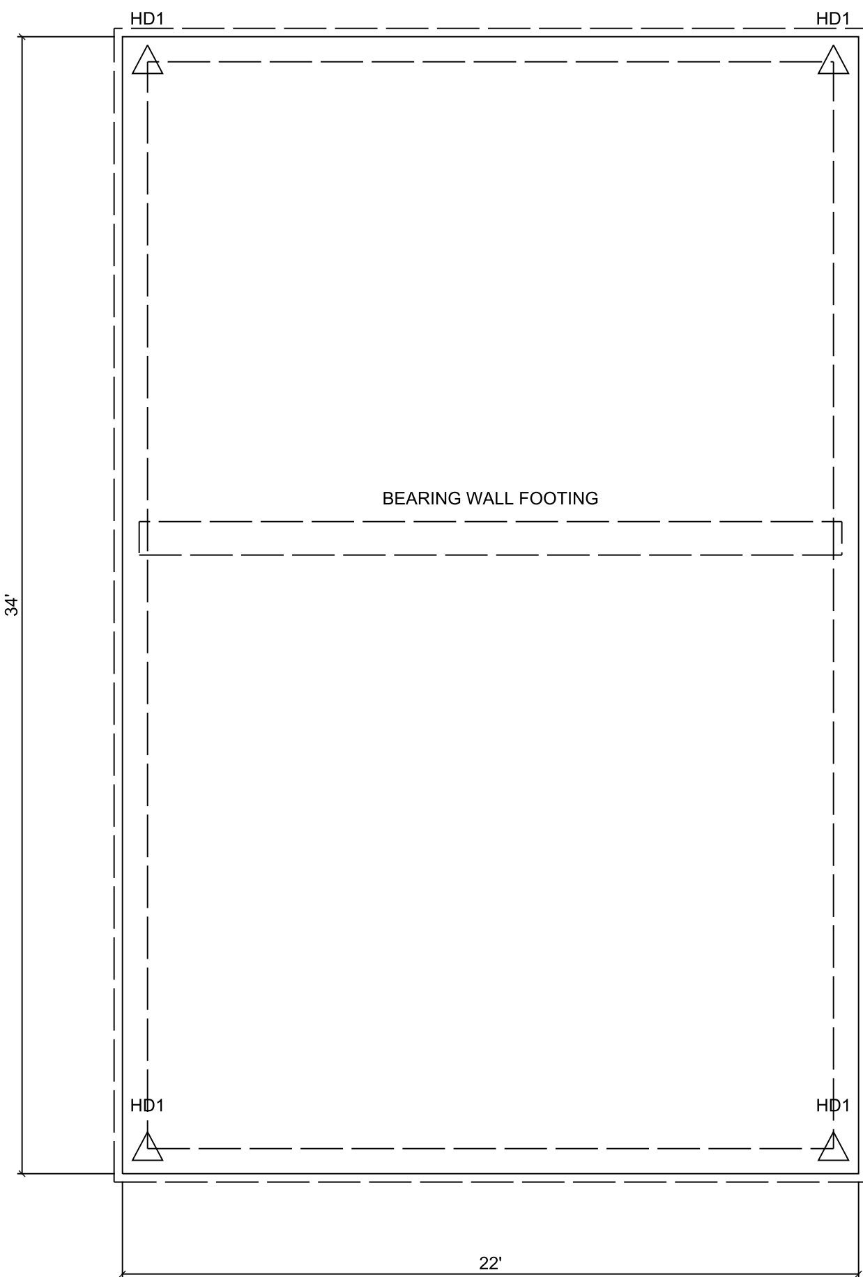
FOUNDATION PLAN
