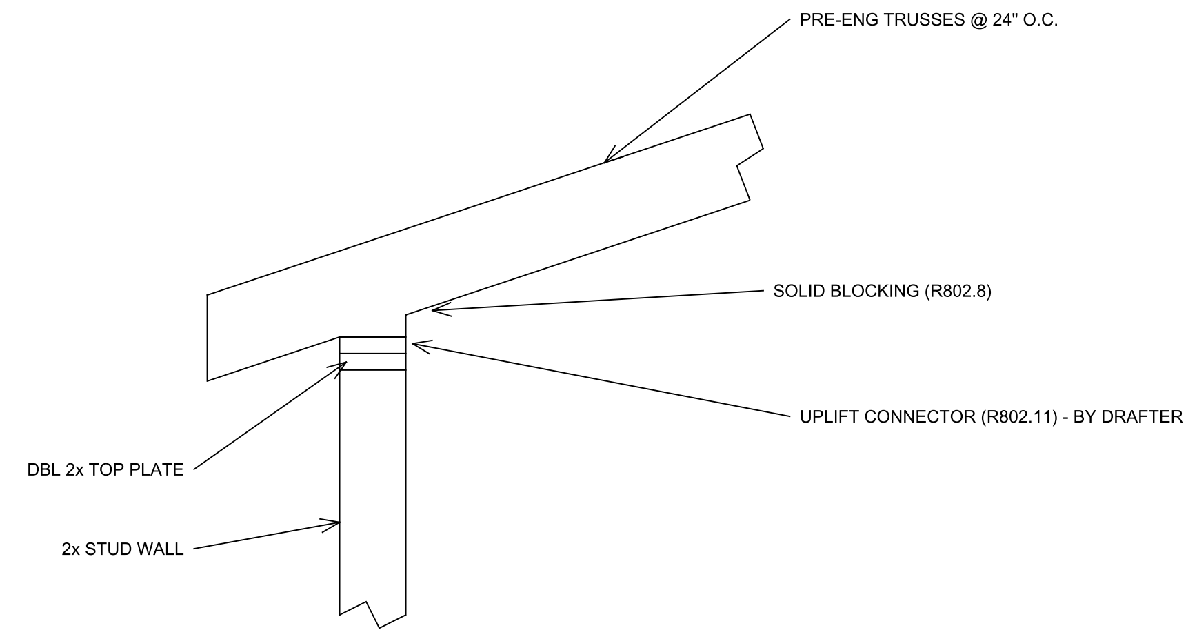
3 EAVE CONNECTION AT TOP PLATE SCALE: 1" = 1'-0"
