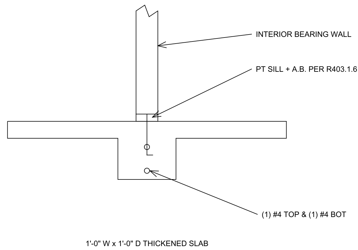
2 INTERIOR BEARING FOOTING SCALE: 1" = 1'-0"
