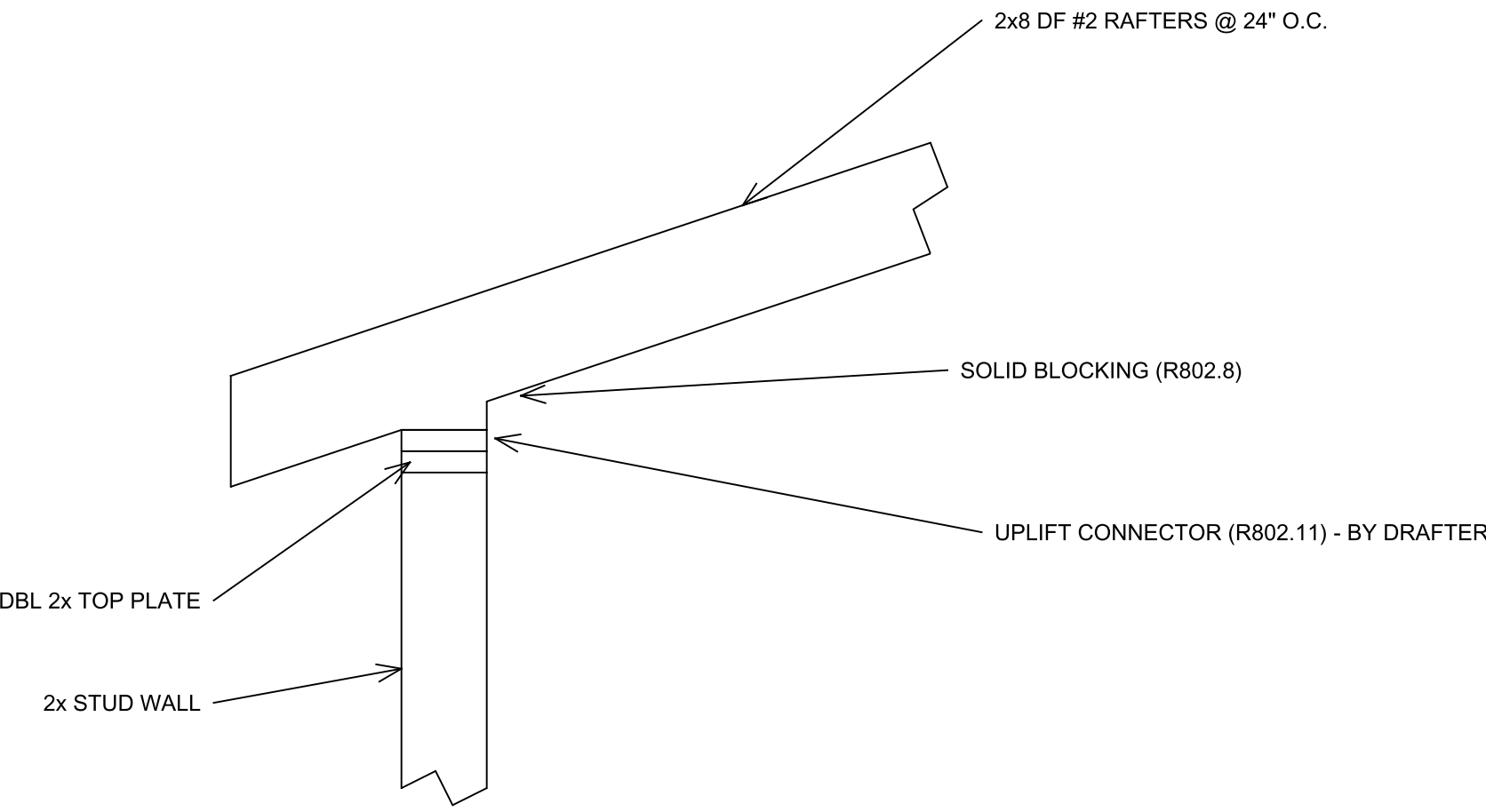
2 EAVE CONNECTION AT TOP PLATE SCALE: 1" = 1'-0"
