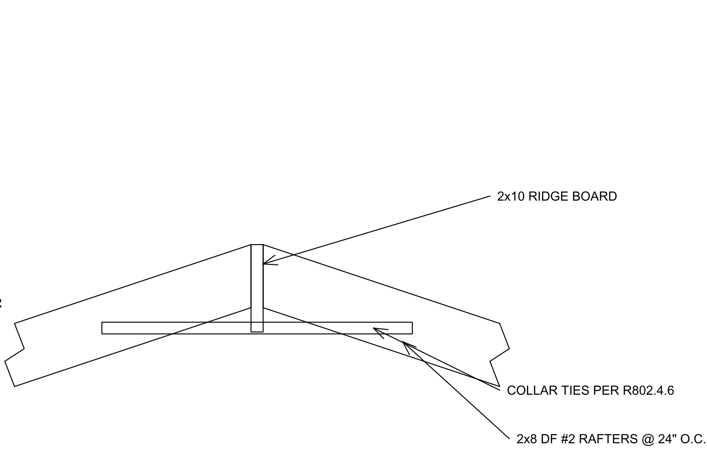
3 RIDGE CONNECTION SCALE: 1" = 1'-0"
