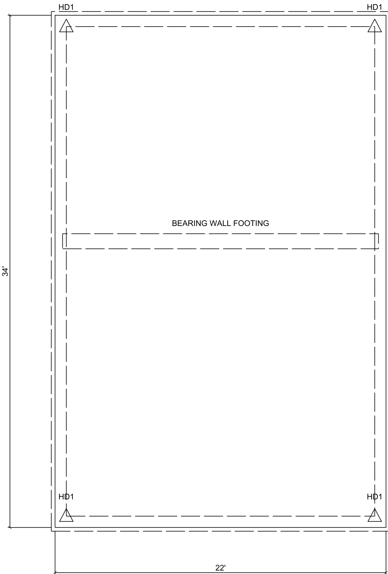
FOUNDATION PLAN
