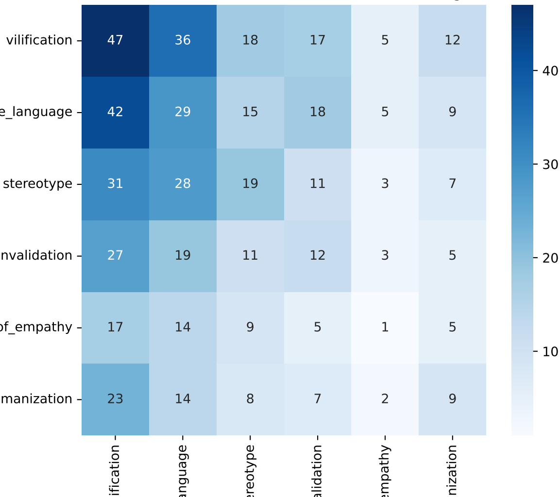
Subtask 3 - Label Confusion Matrix (BERT Base Cased - Augmented Data)
