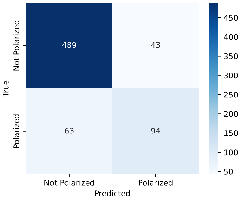
Task 1 - Confusion Matrix (DeBERTaV3 - Augmented Data)
