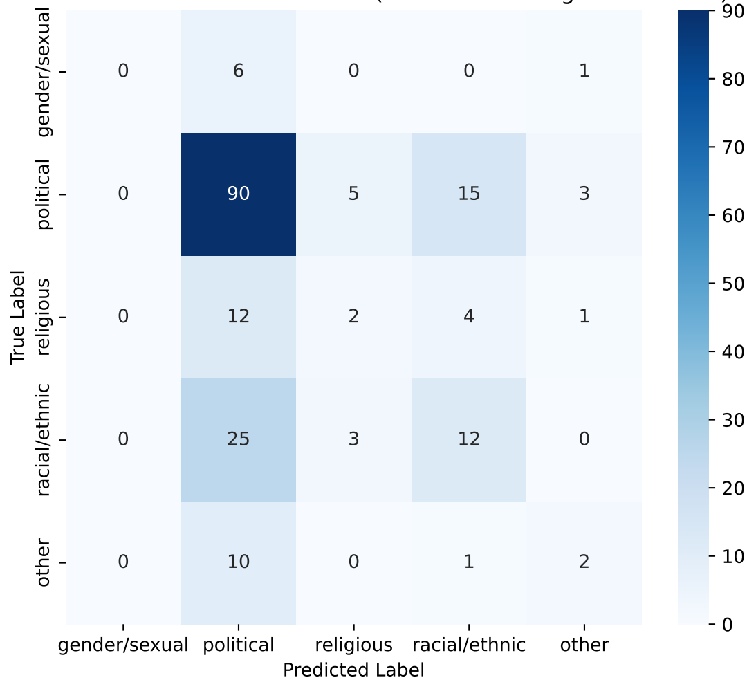
Subtask 2 - Label Confusion Matrix (DeBERTaV3 - Augmented Data)
