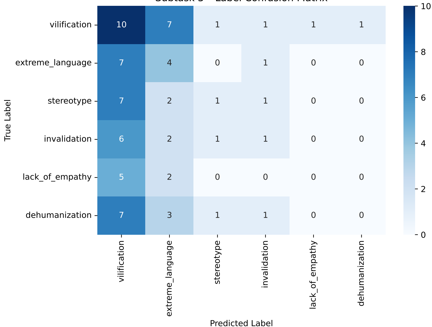
Subtask 3 - Label Confusion Matrix
