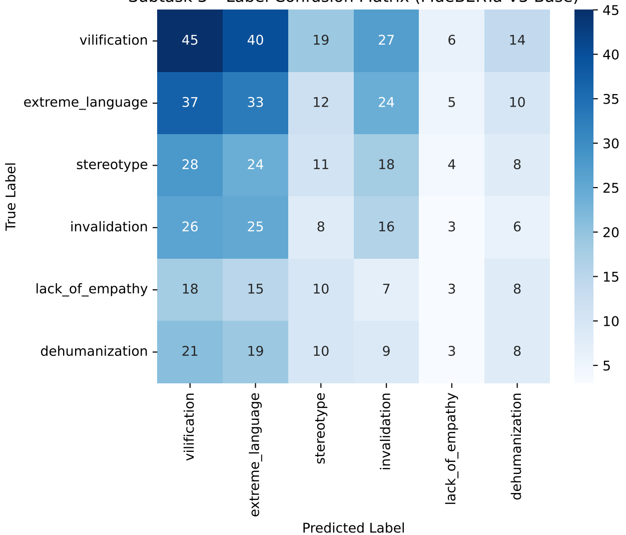
Subtask 3 - Label Confusion Matrix (MdeBERTa V3 Base)
