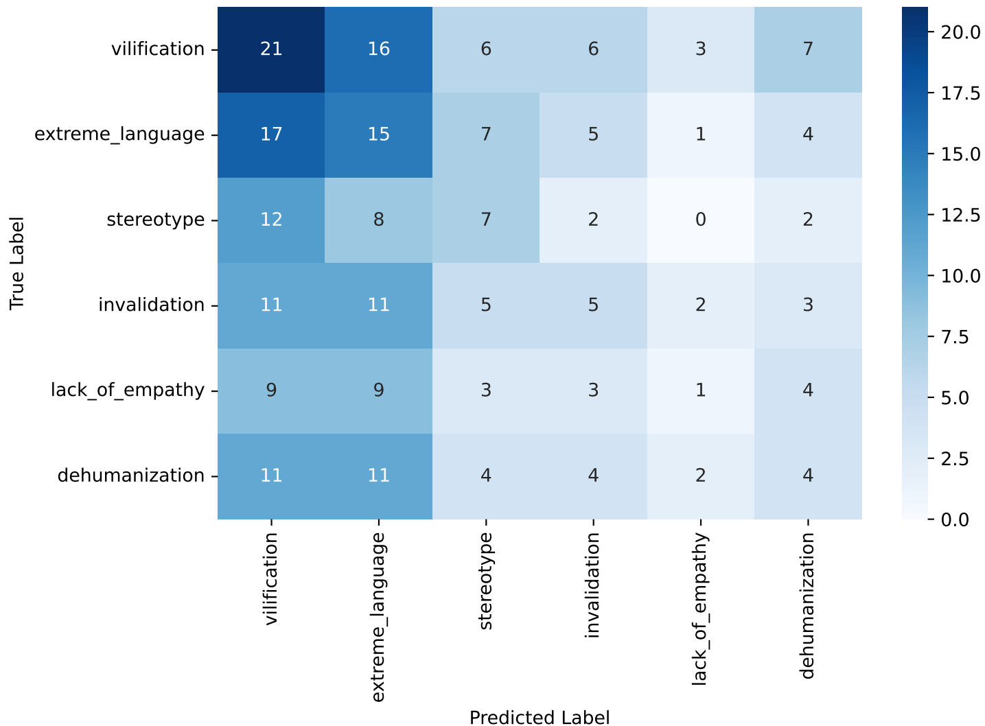
Subtask 3 - Label Confusion Matrix
