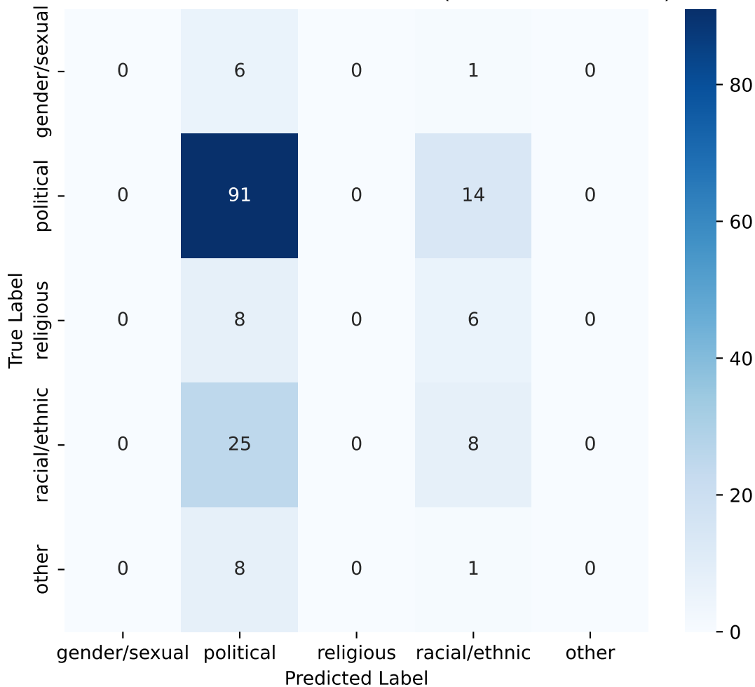
Subtask 2 - Label Confusion Matrix (MdeBERTa V3 Base)
