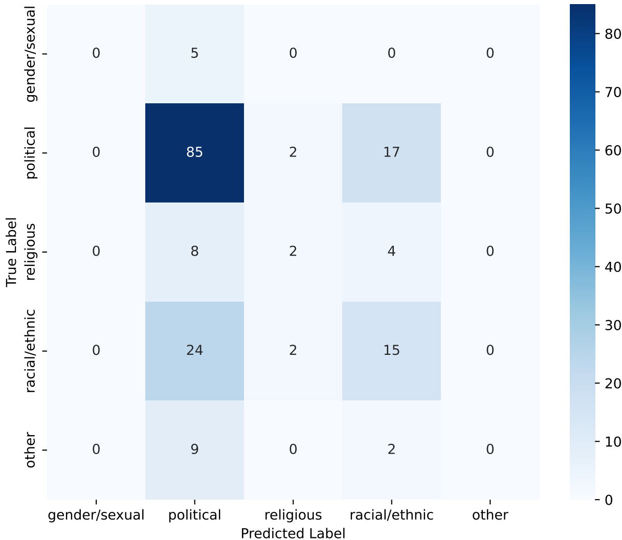
Subtask 2 - Label Confusion Matrix (MdeBERTa V3 Base)
