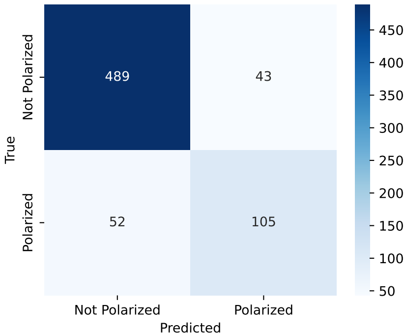
Figure 1 - Confusion Matrix (BERT Base Cased - Augmented Data)
