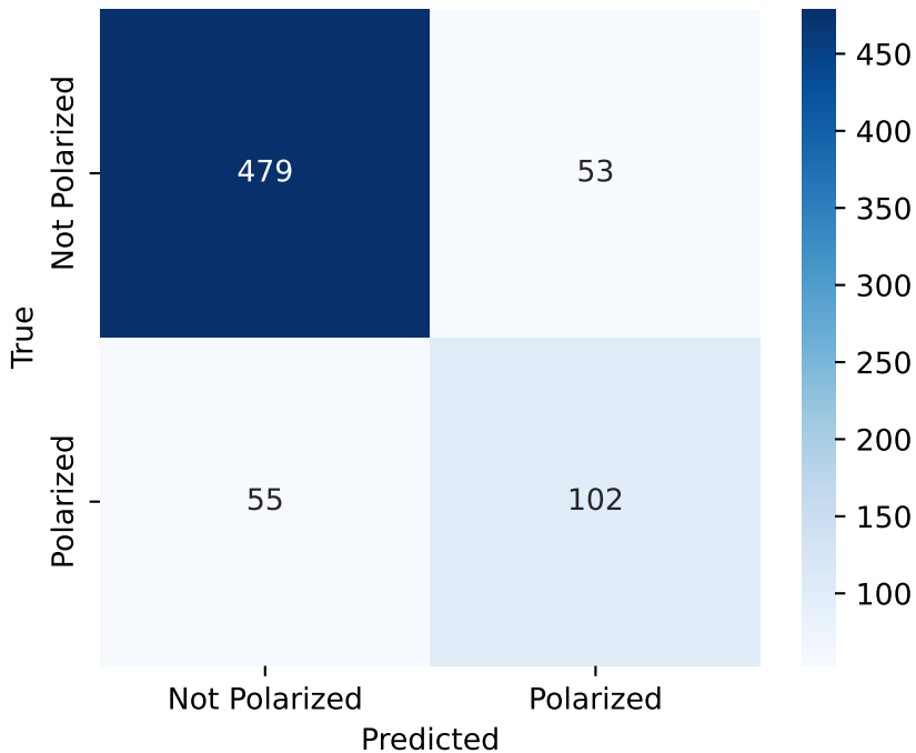
Task 1 - Confusion Matrix (Afro XLMR Base - Augmented Data)
