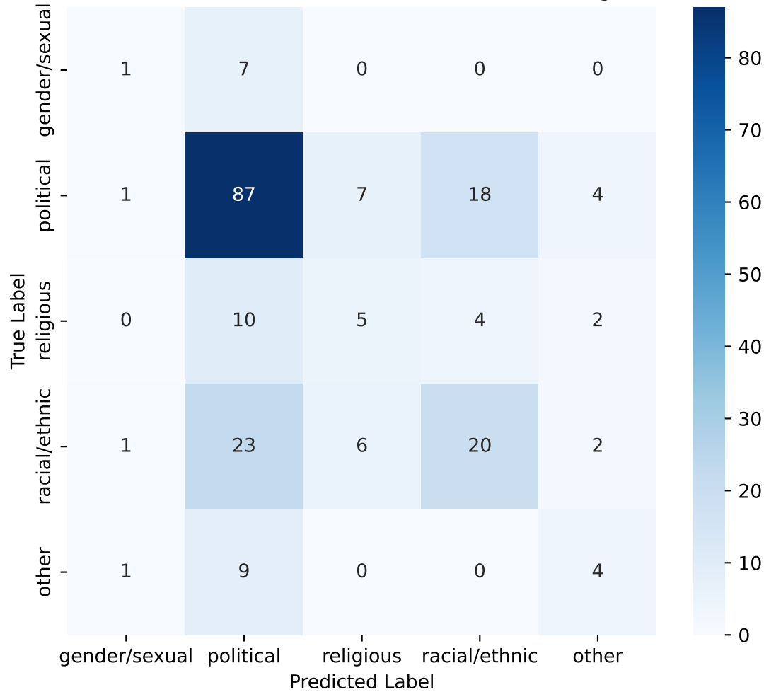
Subtask 2 - Label Confusion Matrix (Afro XLMR Base - Augmented Data)
