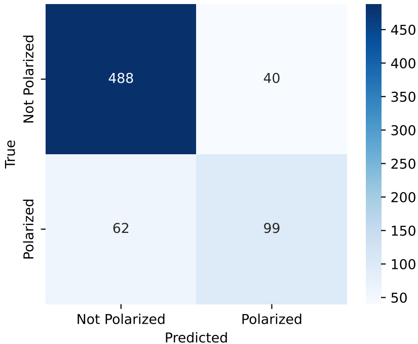
Subtask 1 - Confusion Matrix (Afro-XLMR-Base)
