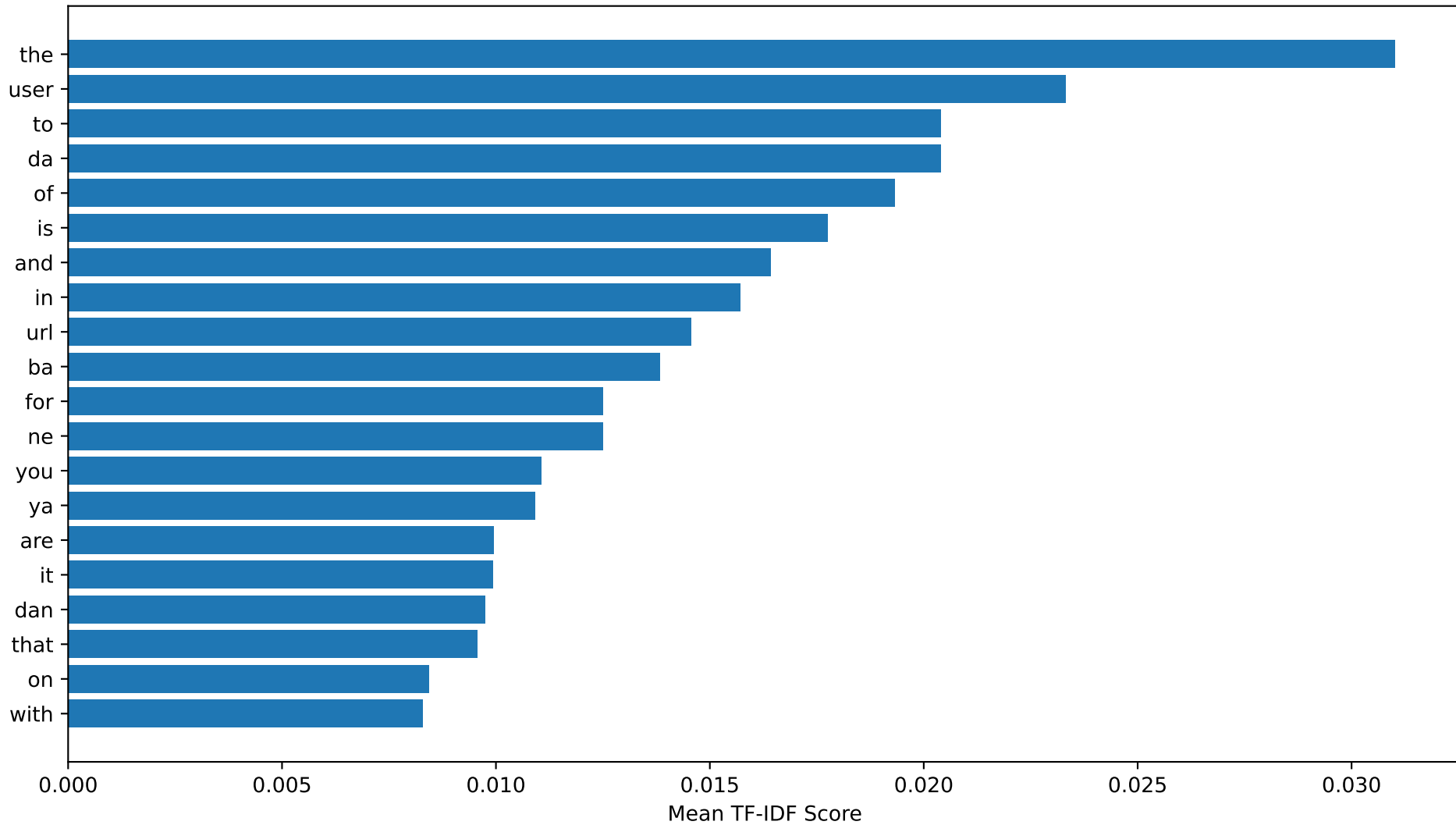
Subtask 1: Most Important Words (TF-IDF)
