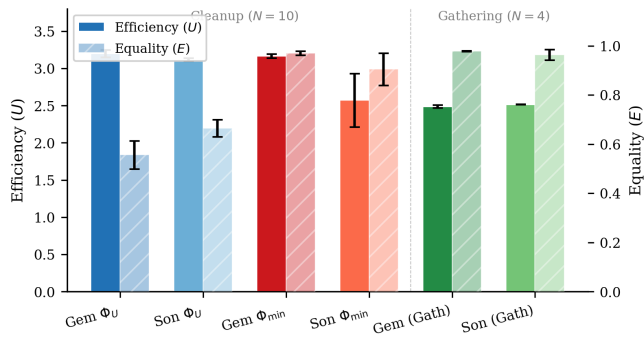
Figure 4: Final efficiency ( U , bars) and equality ( E , hatched bars) for all 12 runs, grouped by condition. Error bars show half-range across 2 runs. Maximin-optimized Gemini runs achieve both high efficiency and near-perfect equality, while efficiency-optimized runs show moderate equality. Gathering runs achieve high equality regardless of objective.
