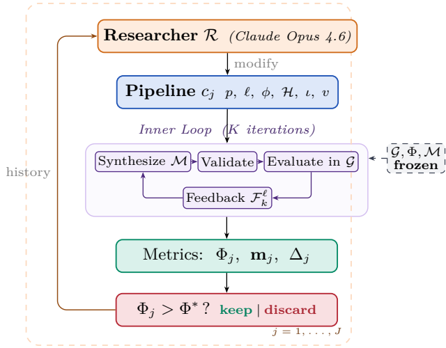
Figure 1: Two-level automated research framework (Algorithm 1). Outer loop : the researcher \mathcal{R} modifies the pipeline configuration c_j , runs the inner loop, and keeps or discards based on \Phi . Inner loop : the policy LLM \mathcal{M} iteratively synthesizes, validates, and evaluates policies in the frozen environment \mathcal{G} .
