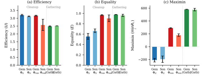
Figure 4: Final metrics across all conditions. (a) Efficiency: all conditions converge to U \approx 2.5 – 3.2 . (b) Equality: maximin-optimized Cleanup runs achieve E \approx 1.0 , while efficiency-optimized runs show E \approx 0.5 – 0.7 ; Gathering achieves high equality regardless. (c) Maximin: the sharpest contrast—efficiency optimization leaves the worst-off agent deeply negative ( \min_i R_i \approx -200 ), while maximin optimization transforms it to +290 (Gemini) or +179 (Sonnet). Gathering achieves high maximin ( \sim 580 ) under efficiency optimization alone. Error bars show s.d. across runs.
