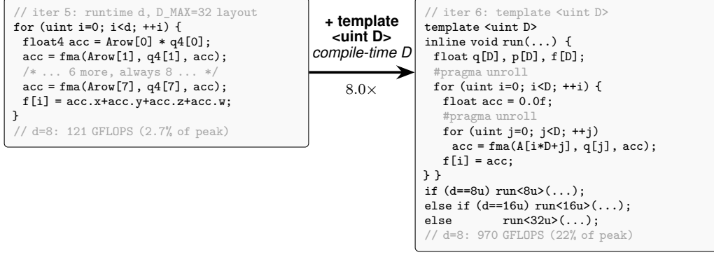
Figure 1: Paradigmatic candidate evolution: HMC, Opus 4.7, iter 5 \rightarrow 6. Both Opus and Pro independently arrive at this structural change. The lever is one declaration — template <uint D> with runtime-dispatched instantiations on d . Iter 5 had a manually-unrolled float4 inner loop against a fixed D_{\max}=32 layout (over-computing at d=8 , plus a 4-way horizontal sum); iter 6 sizes q, p, f exactly to D so both loops fully unroll into scalar FMAs — moving d=8 from 121 to 970 GFLOPS in one iteration after five had stalled at 2–4% of peak. Opus enumerated D \in \{8, 16, 32\} and broke correctness at the held-out d=24 ; Pro kept a runtime- d fallback and generalised cleanly.
