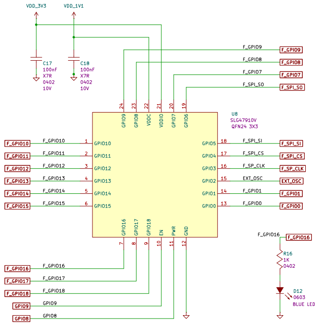
FPGA SLG47910
