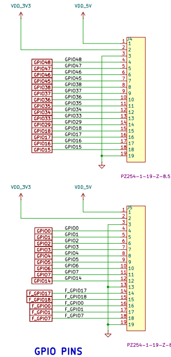
GPIO PINS
