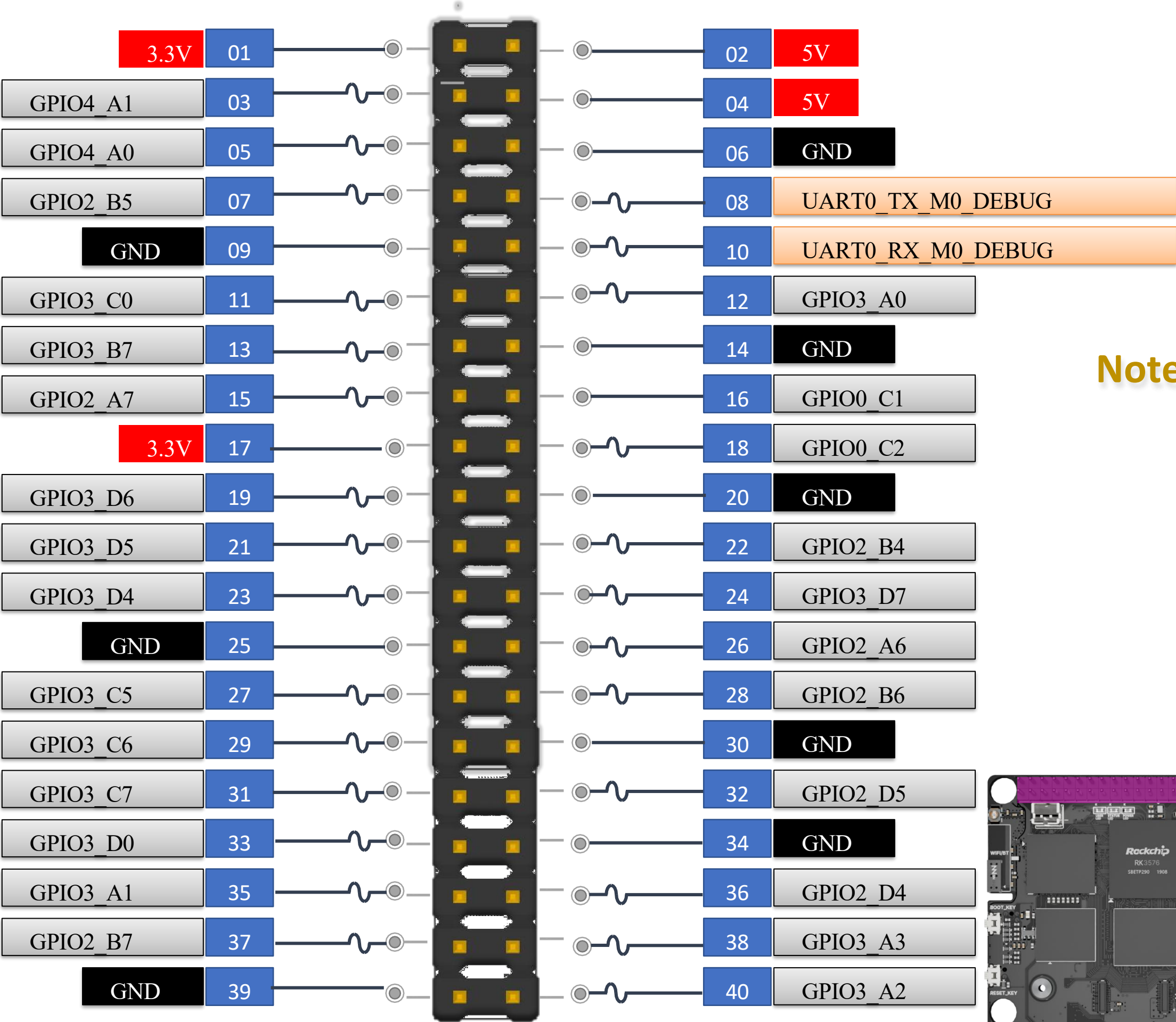
RK3576 40Pin GPIO Header 2.54mm
