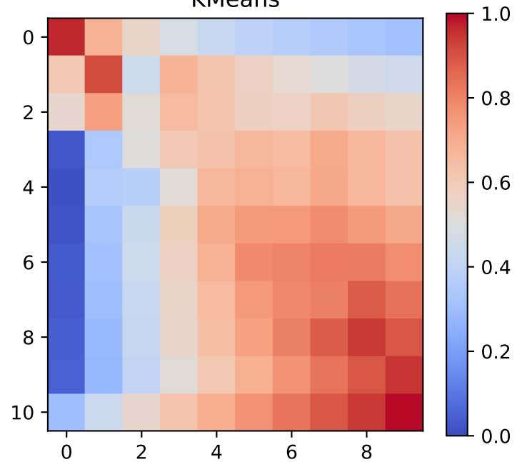
KMeans
