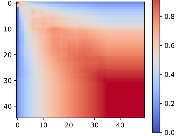
KMeans
