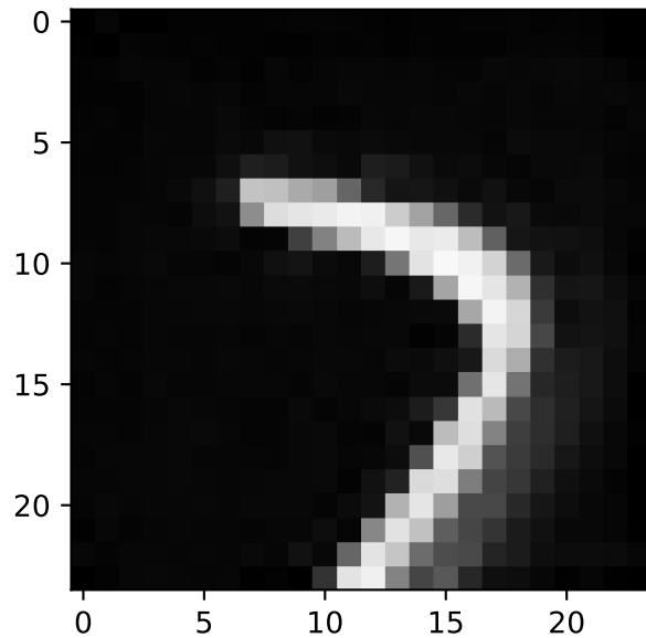
(561,2)
