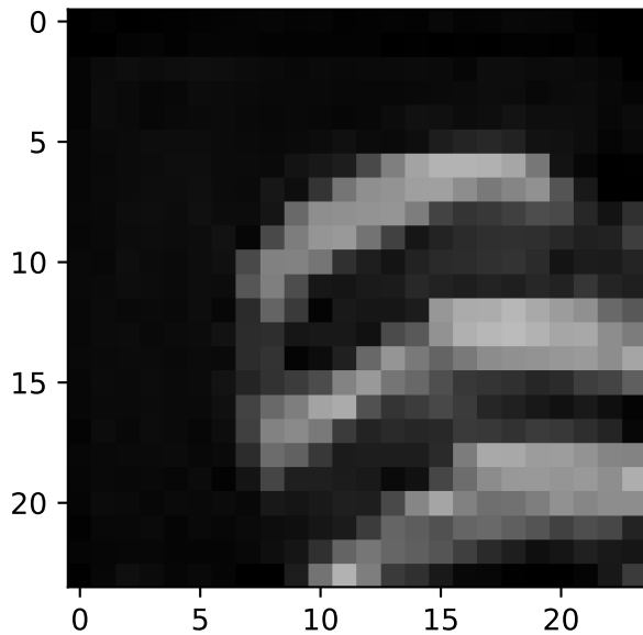
(561,0)
