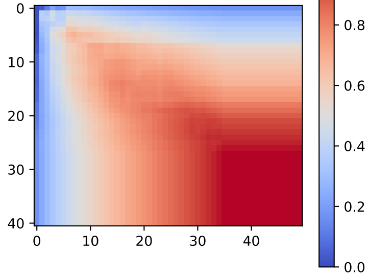
KMeans
