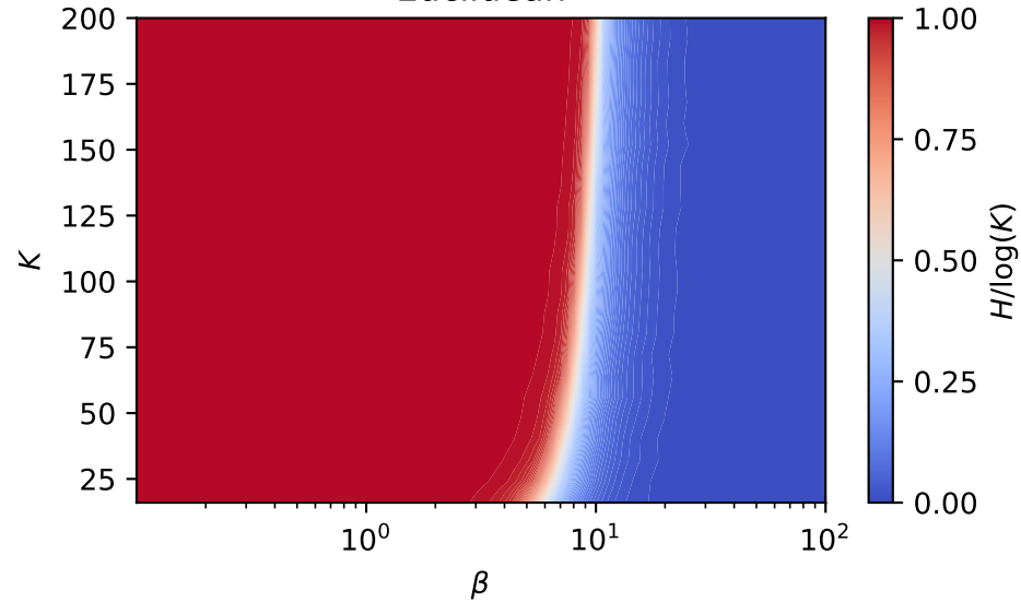
Euclidean
