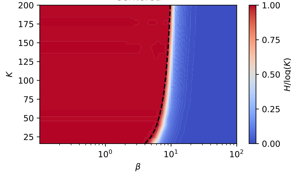
Centered
