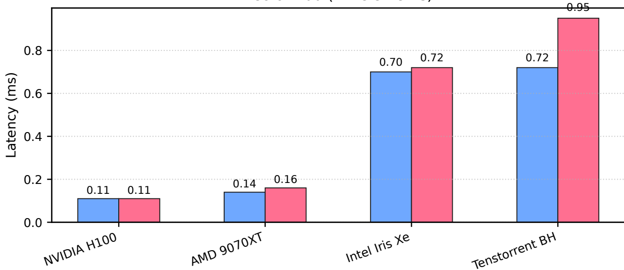
Vendor Baseline Concordi Vector Add (1M elements)
