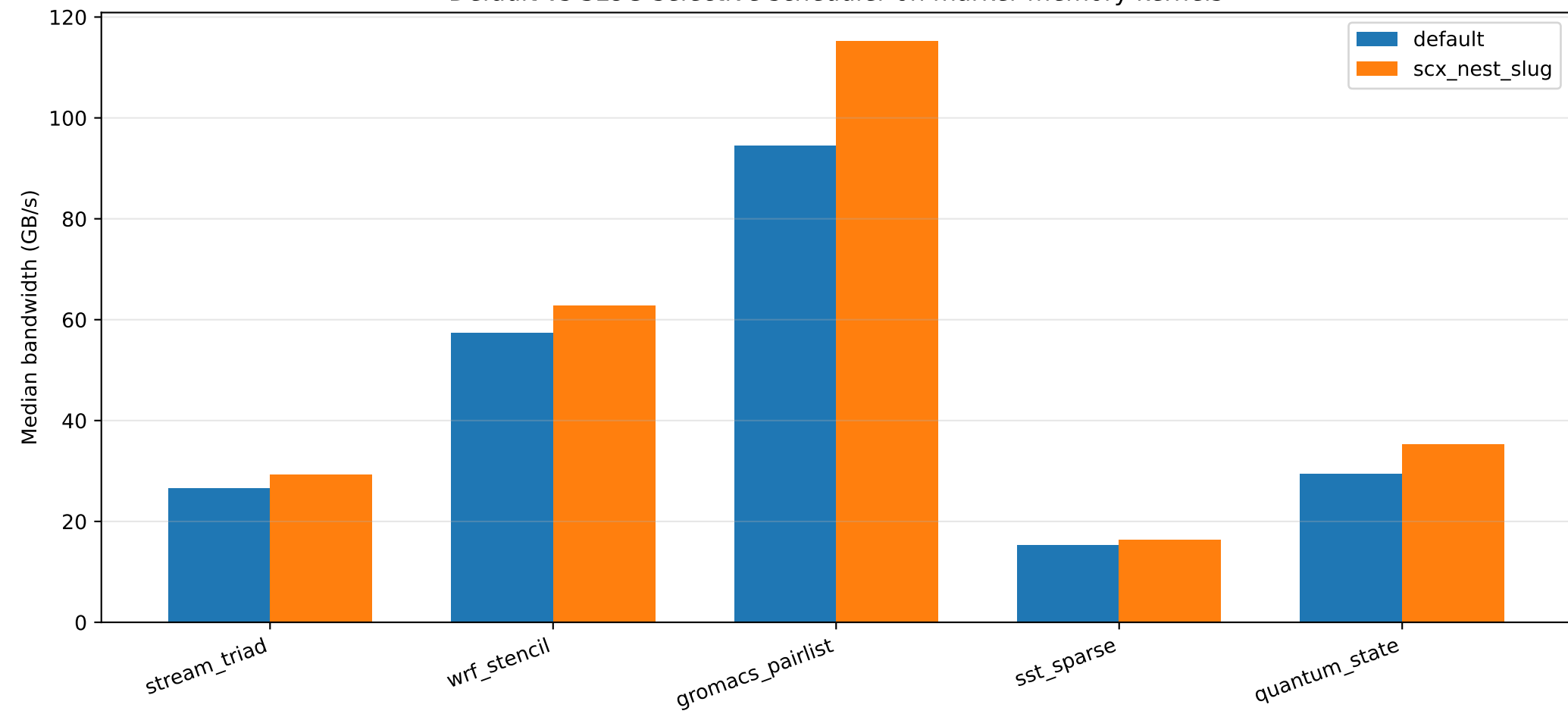
Default vs SLUG-selective scheduler on marker memory kernels
