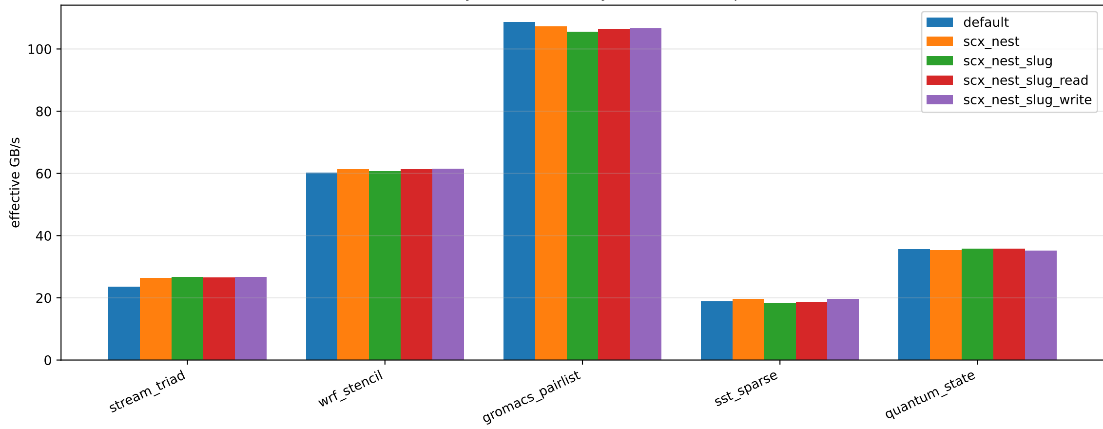
HPC Memory-Bandwidth Proxy Scheduler Comparison
