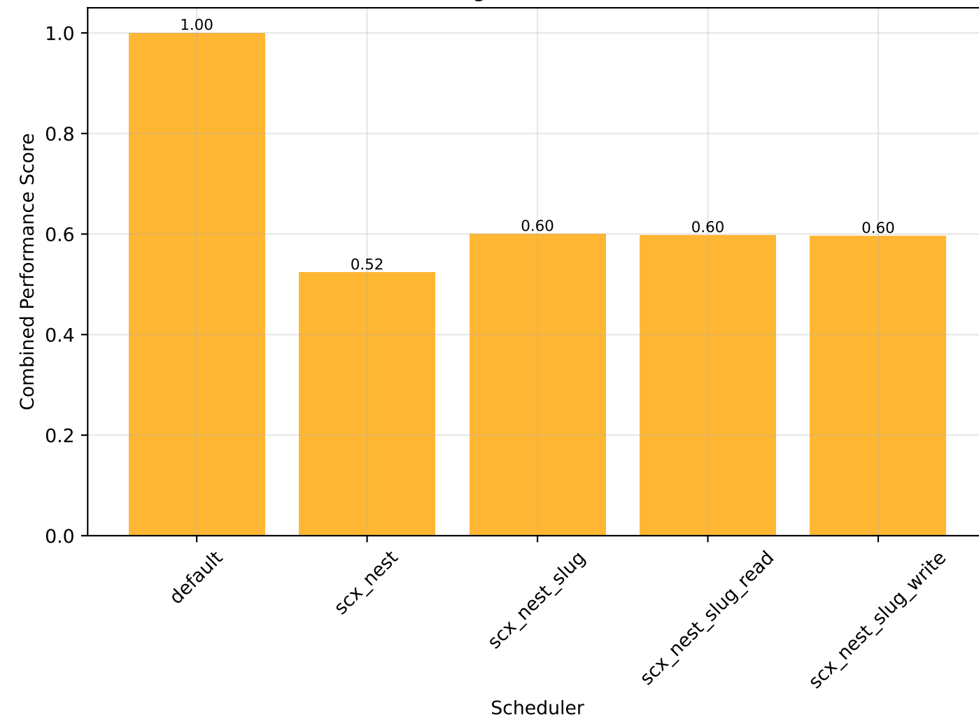
Overall Performance Score (Higher is Better)
