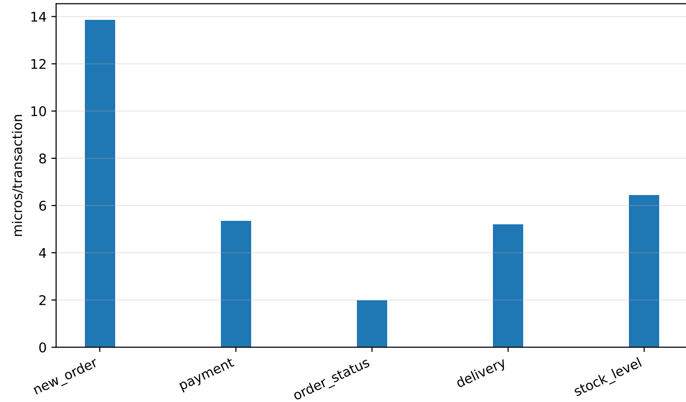
Per-Query Latency
