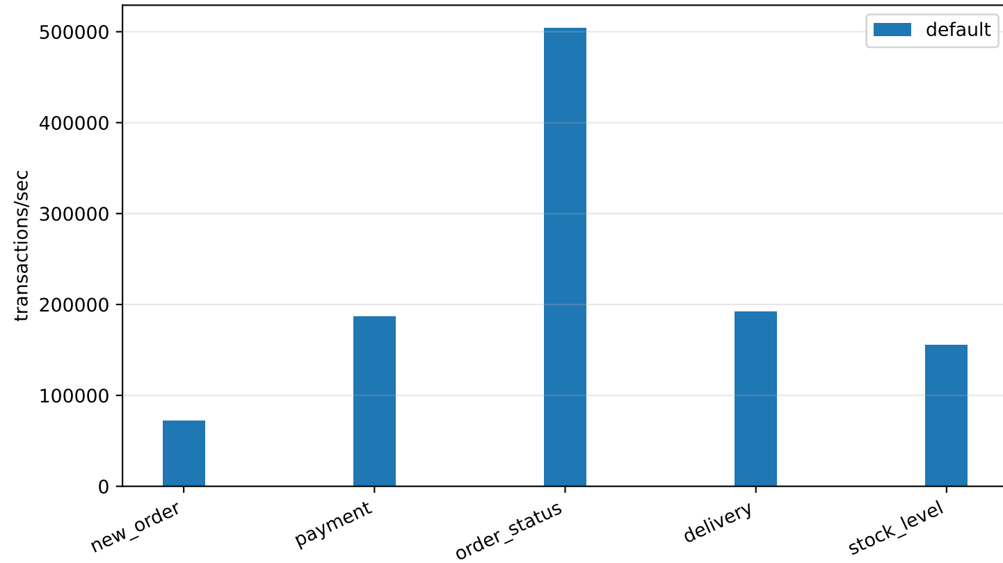
Per-Query Throughput
