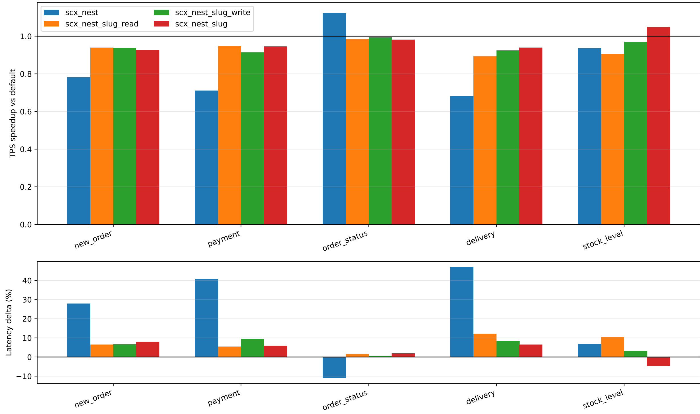
RocksDB TPCC-like traces: scheduler speedup
