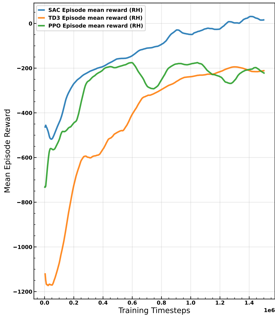
RehabBot Mean Episode Reward (RH)
