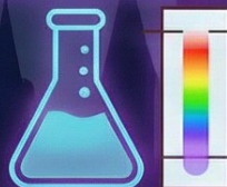
Day 2: 墨水分析 (Ink Chromatography)
