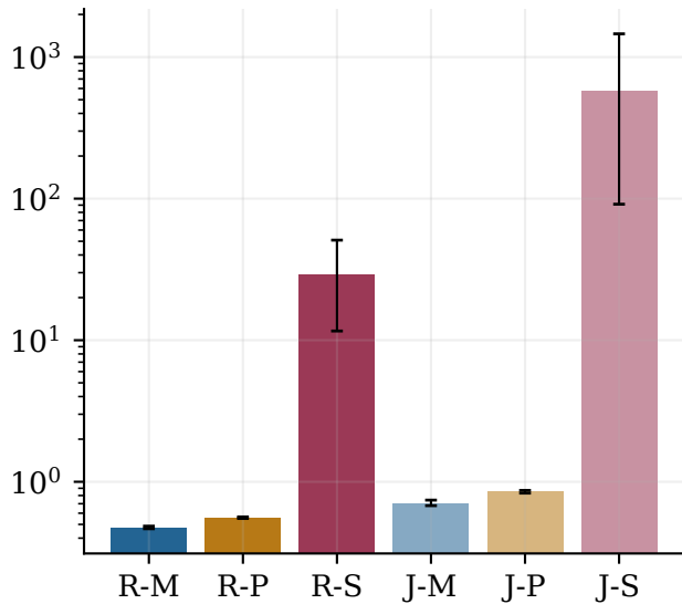
Mean within-run publish p99 (ms)
