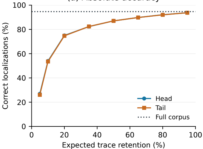
(a) Absolute accuracy
