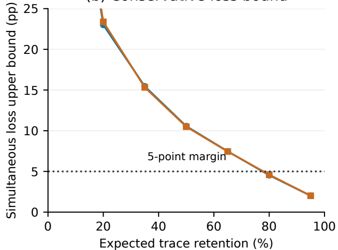
(b) Conservative loss bound
