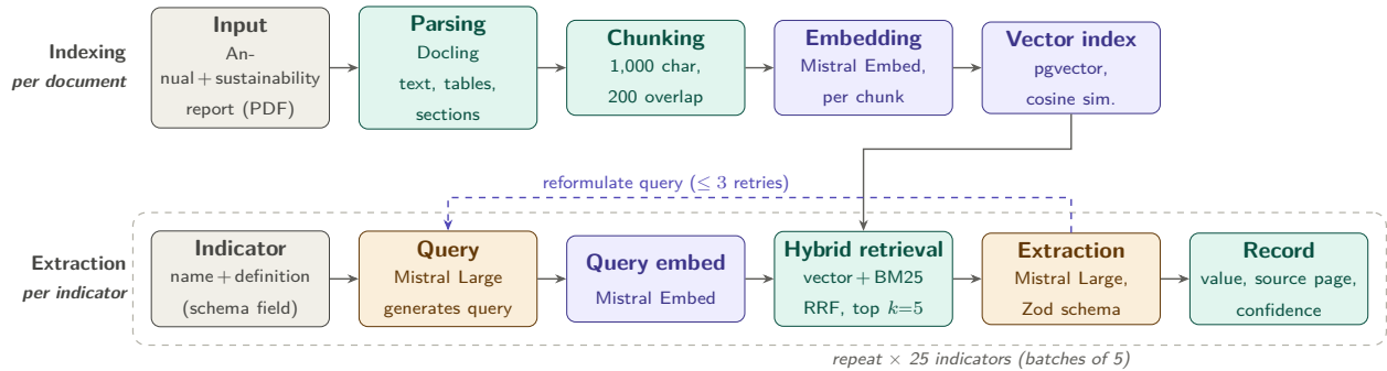
Figure 1: ESG extraction pipeline. Top lane: one-off indexing per document. Bottom lane: per-indicator extraction, repeated for all 25 indicators (batches of five); the dashed arrow marks the query-reformulation retry loop.
