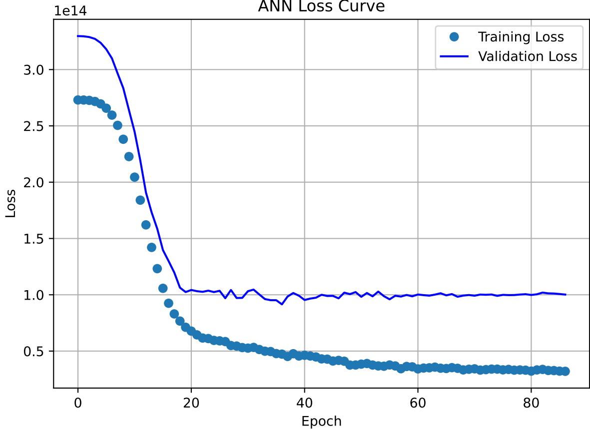
ANN Loss Curve
