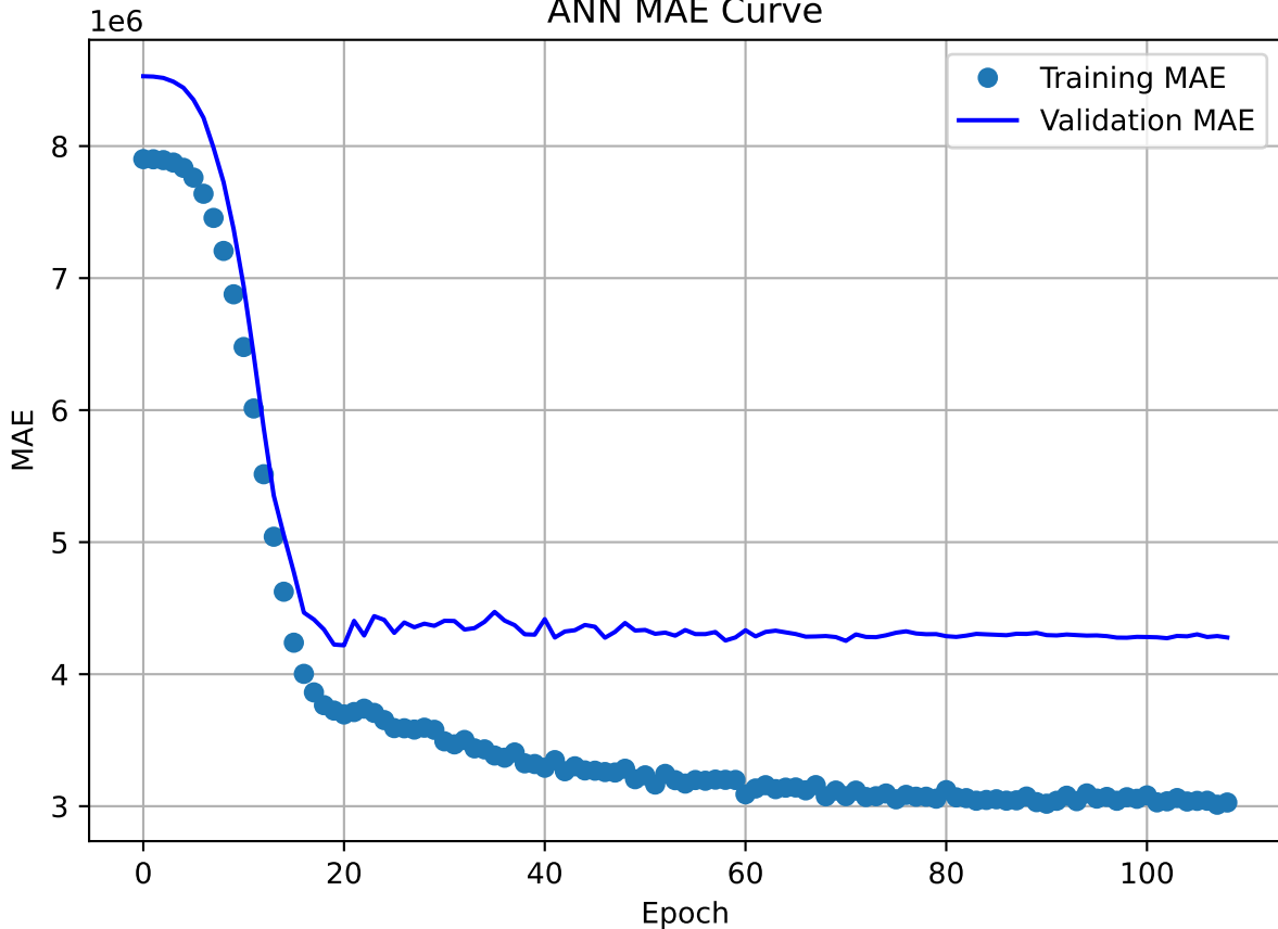
ANN MAE Curve
