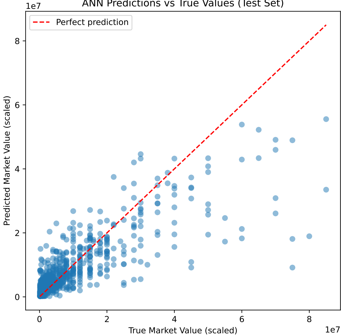
ANN Predictions vs True Values (Test Set)
