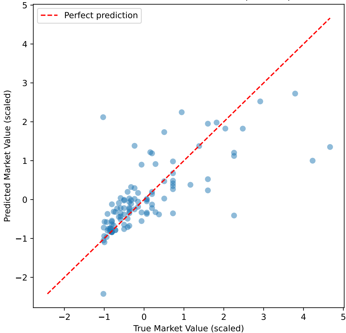
ANN Predictions vs True Values (Test Set)
