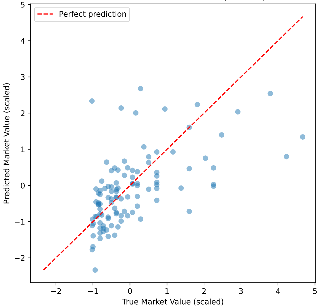
OLS Predictions vs True Values (Test Set)
