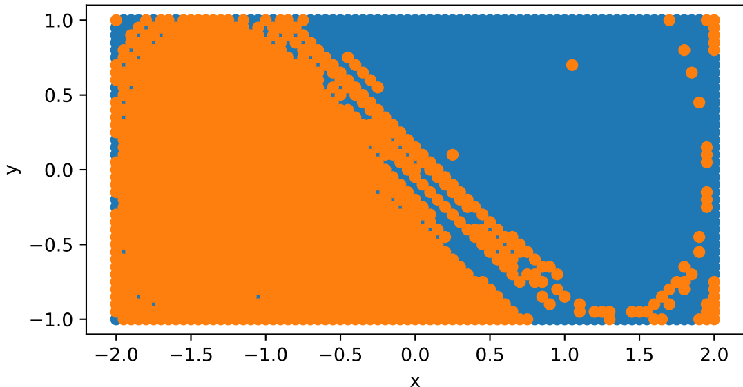
Clusters
