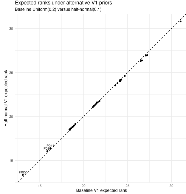
Figure 12: Posterior expected ranks under the baseline V1 prior specification and the half-normal prior-sensitivity specification. The dashed identity line represents identical expected ranks under both models.
