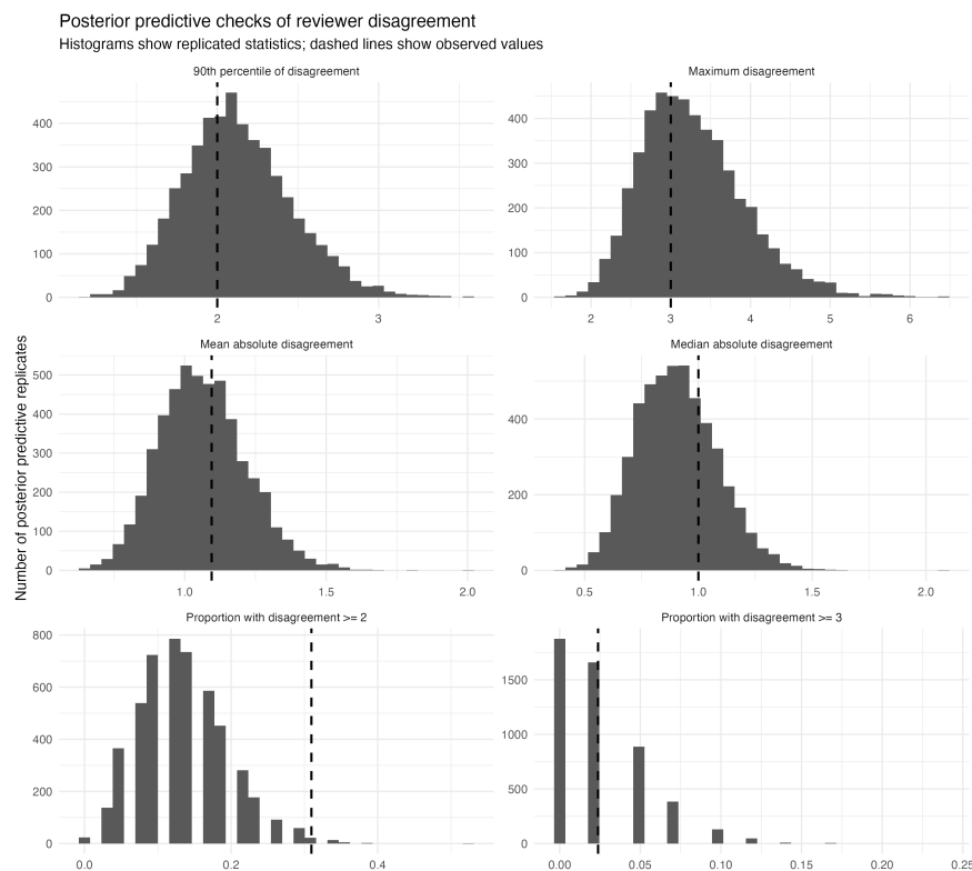
Figure 11: Posterior predictive checks for several summaries of reviewer disagreement under V1. Histograms show statistics from replicated datasets and dashed vertical lines show the corresponding observed values.
