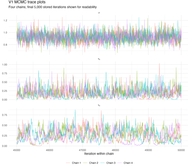
Figure 10: Trace plots for the V1 scale parameters \tau_\theta , \tau_b , and \sigma .
