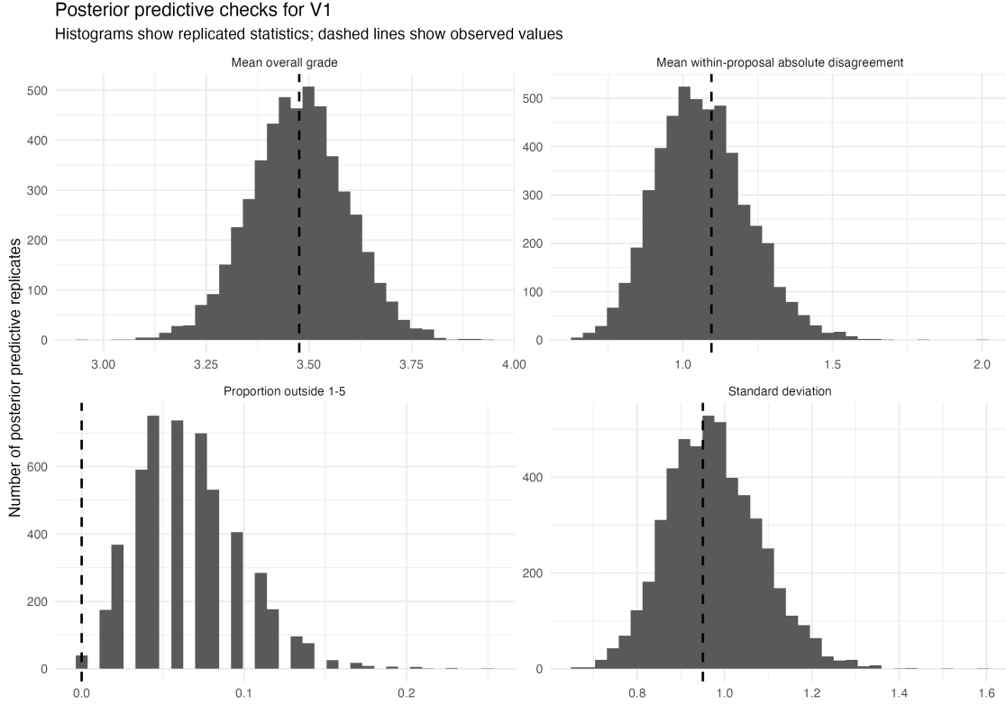
Figure 7: Posterior predictive checks for V1. Histograms show the distributions of statistics calculated from replicated datasets, while dashed vertical lines show the corresponding observed values.
