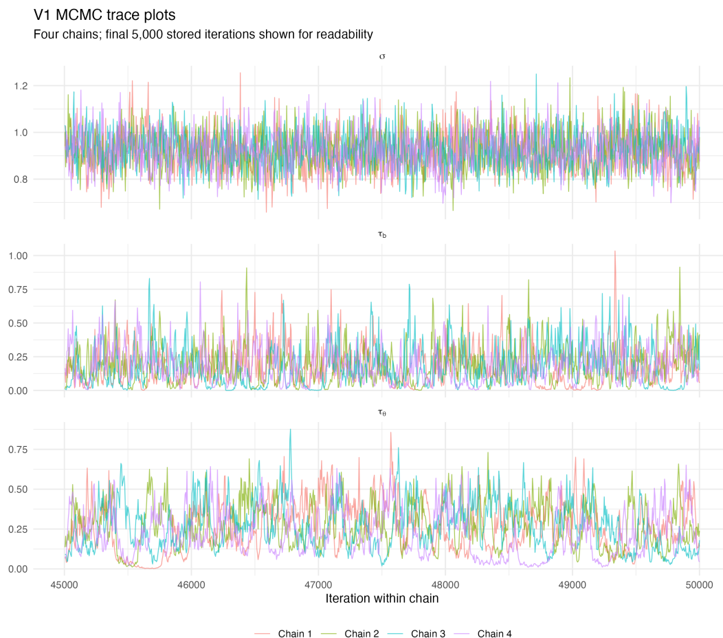
Figure 5: Trace plots for the V1 scale parameters \tau_\theta , \tau_b , and \sigma . The four chains overlap throughout the displayed sampling period without persistent trends or chain separation.
