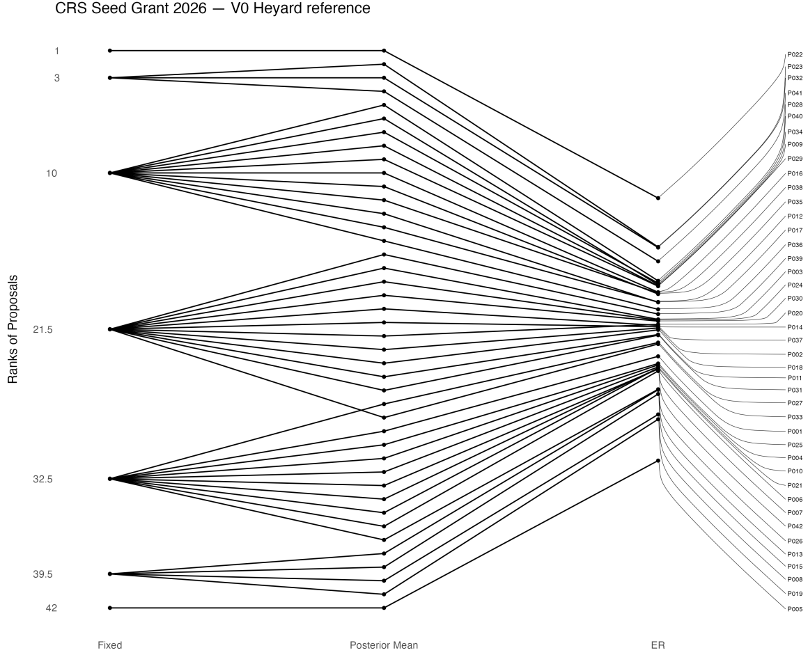
Figure 3: Proposal rankings under the observed-score ranking, posterior-mean ranking and posterior expected rank for the V0 Heyard reference model.
