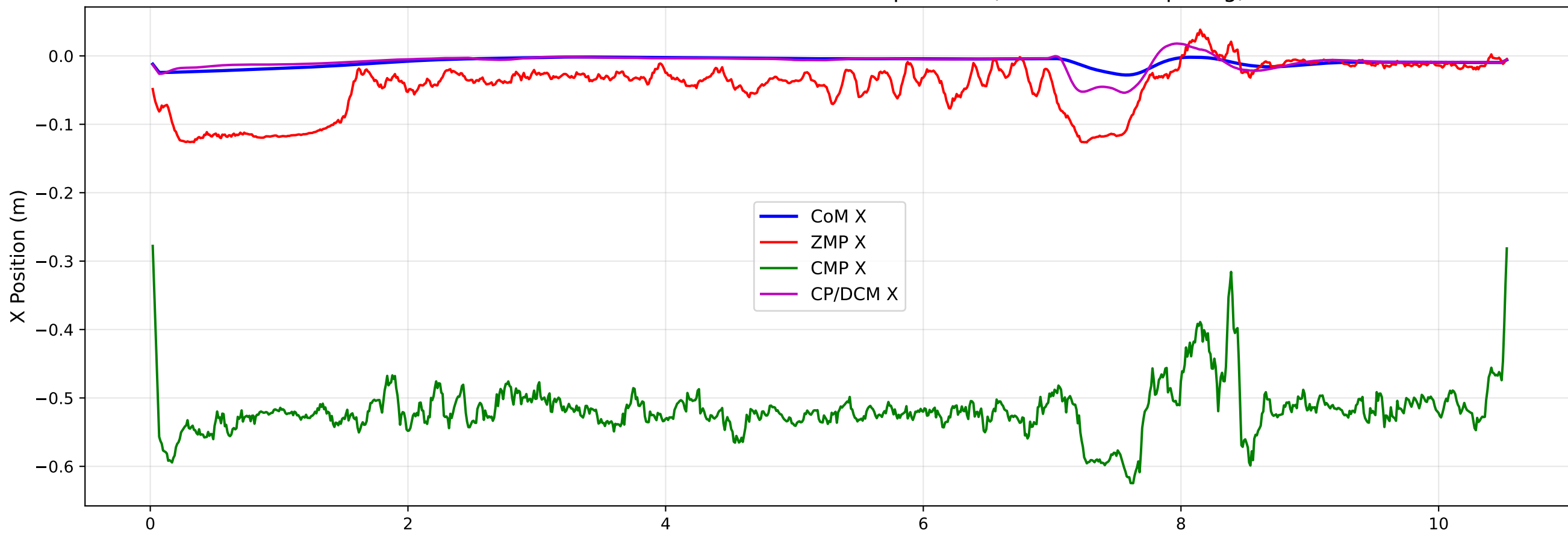
Ground Reference Points and CoM - X Components (Smoothed - 10pt avg)
