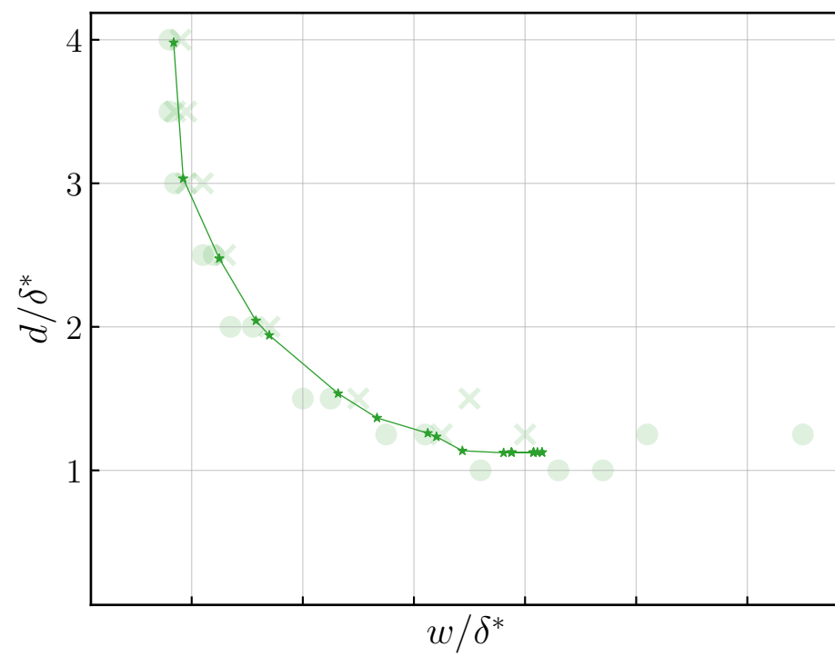
Inc. Re = 3000 2d
