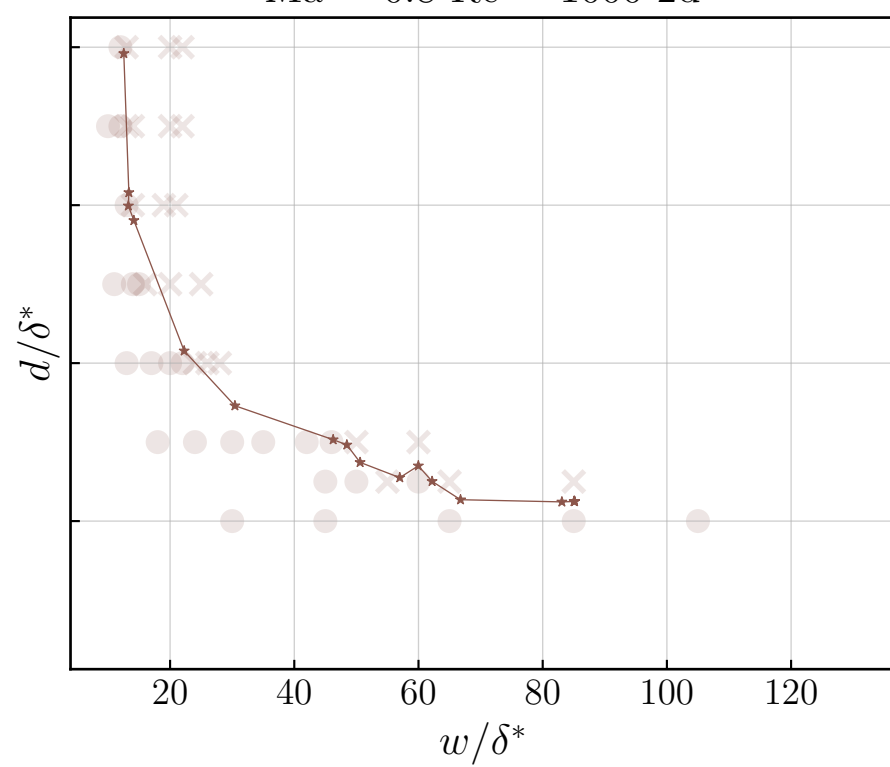
Ma = 0.8 Re = 1000 2d
