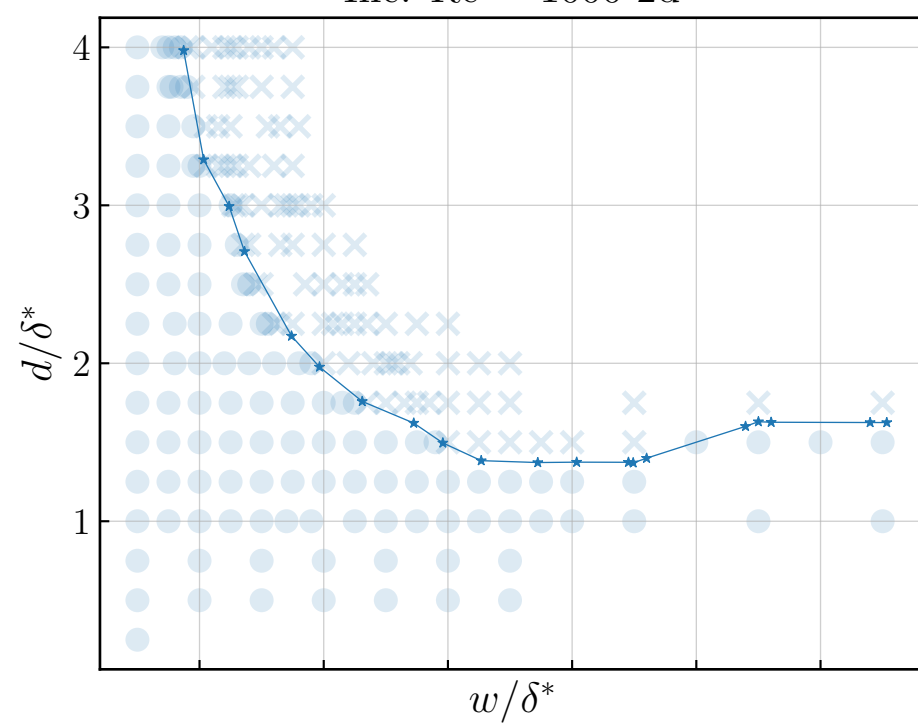
Ma = 0.2 Re = 1000 2d
