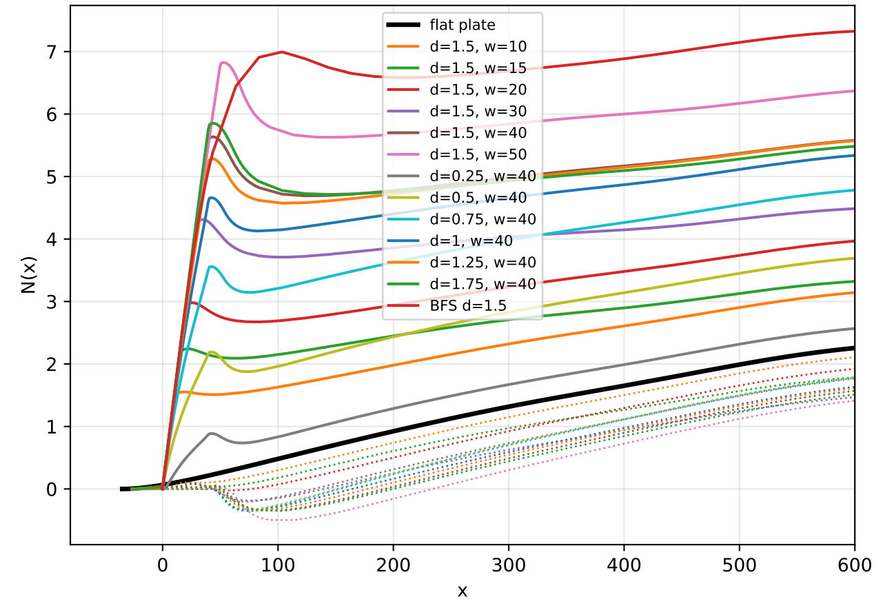
Re = 1000: local theory (dotted: gap contribution removed)
