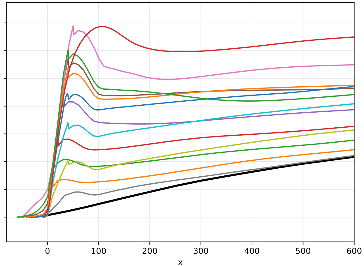
Re = 1000: DNS
