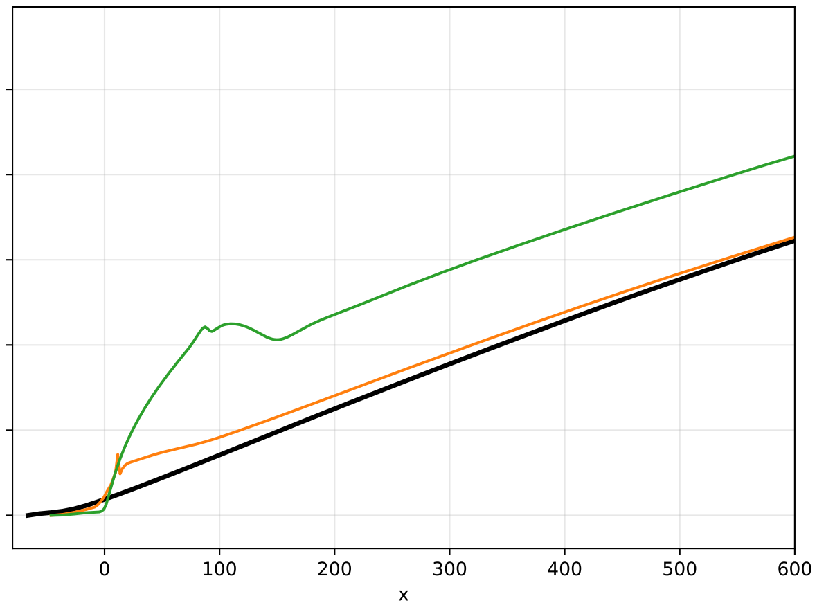
Re = 3000: DNS
