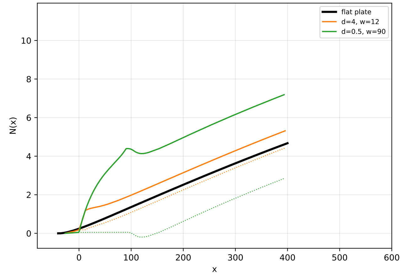
Re = 3000: local theory (dotted: gap contribution removed)
